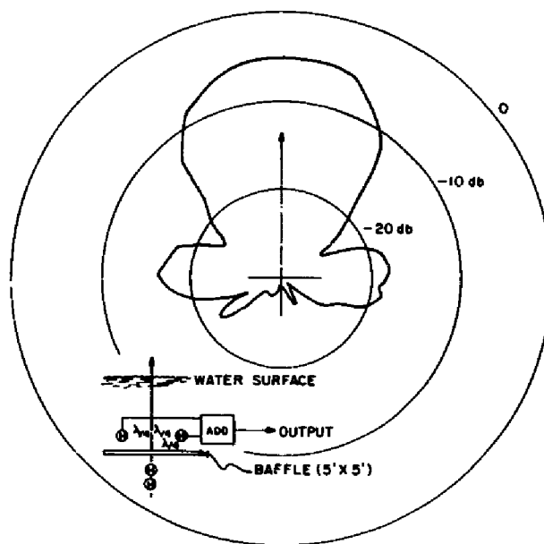
Fig. 1c - Vertical beam pattern noise array 2.3 kc
