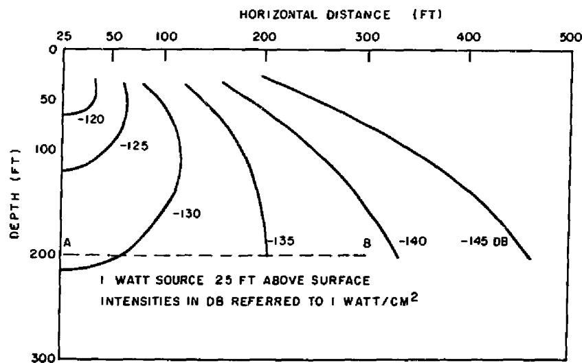
Fig. 18 - Iso-intensity lines versus range and depth for a simple source above an air-water interface.
