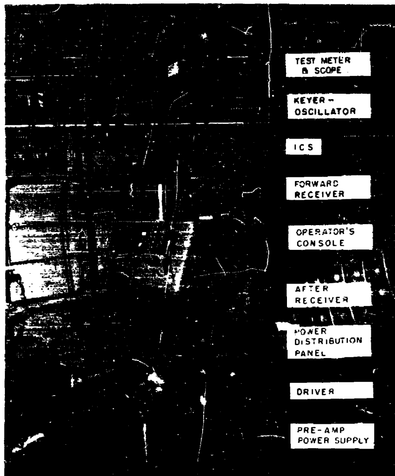
Fig. 6 - Rack I installation
