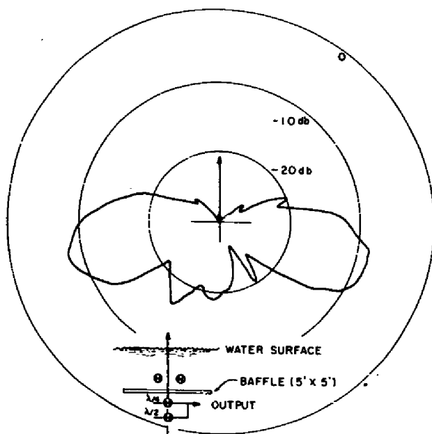
Fig. 1a - Vertical beam pattern noise array (broad null) 2.3 kc
