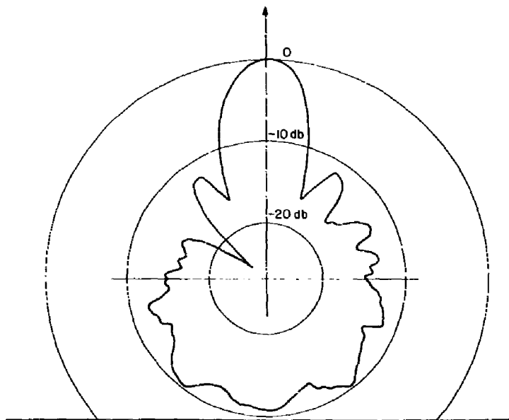
Fig. 15 - 2.3-kc lens pattern with omnidirectional hydrophone
