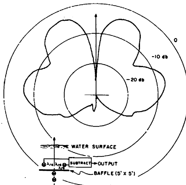
Fig. 1b - Vertical beam pattern noise array (sharp null) 2.3 kc
