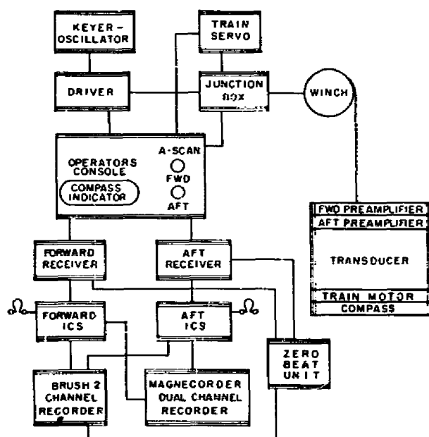
Fig. 5 - Block diagram of LOMASS I system
