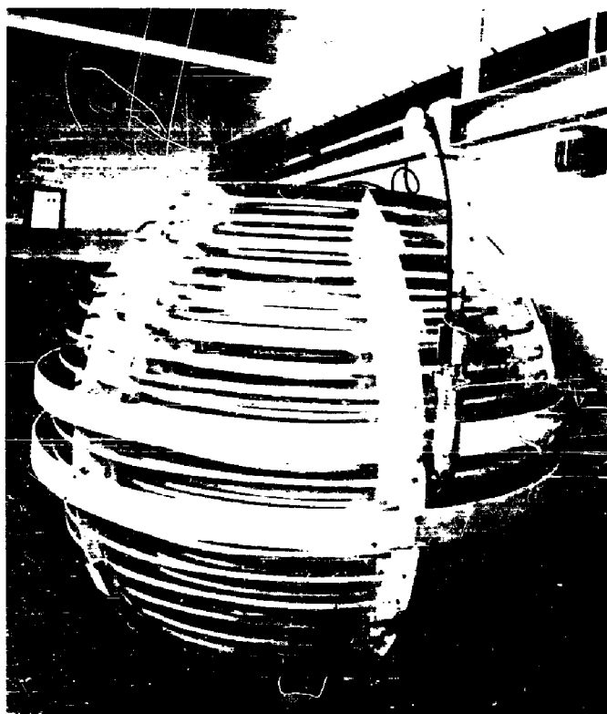
Fig. 13 • Compliant tube receiving lens with mounted hydrophone
