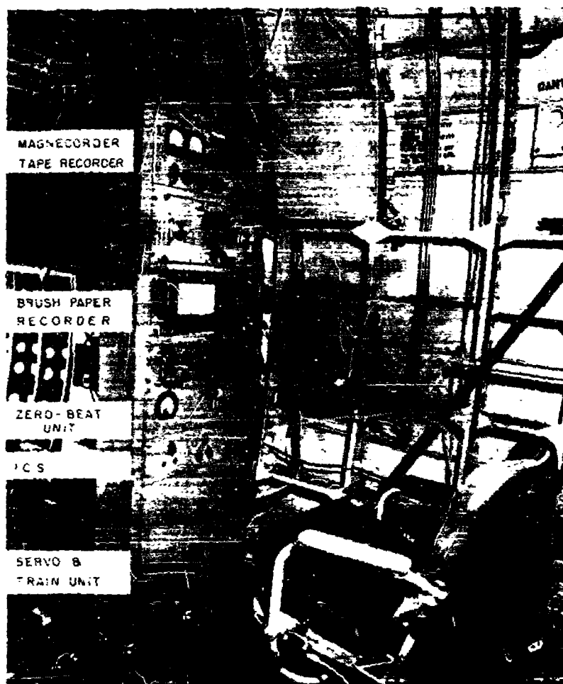
Fig. 7 - Rack II installation
