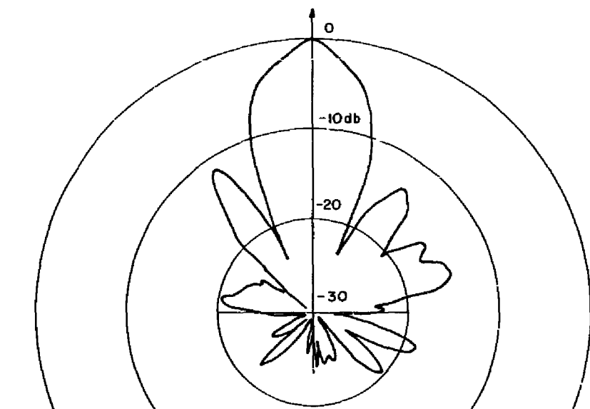
Fig. 16 - 2.3-kc lens pattern with directional hydrophone
