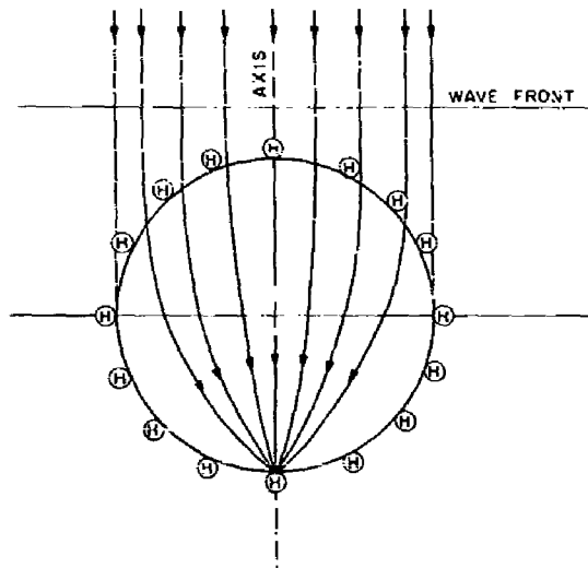
Fig. 14 - Ray diagram of lens operation
