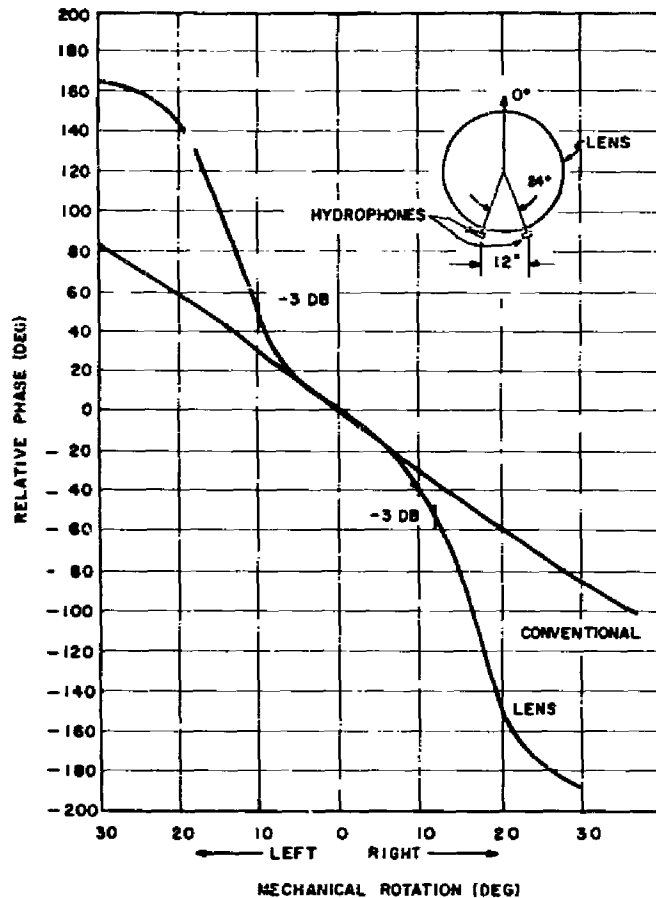
Fig. 17 - Lens phase test
