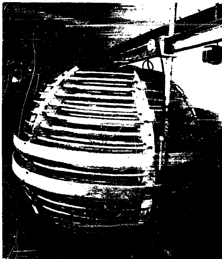
Fig. 13 - Compliant tube receiving lens with mounted hydrophone
