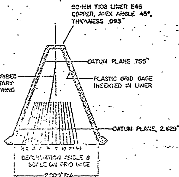
FIGURE 2c - SIDE SECTIONAL VIEW OF ROTARY EXTRUDED LINER. LINER EXHIBITS SPIN ANGLE OF 0° IN A LINE.
