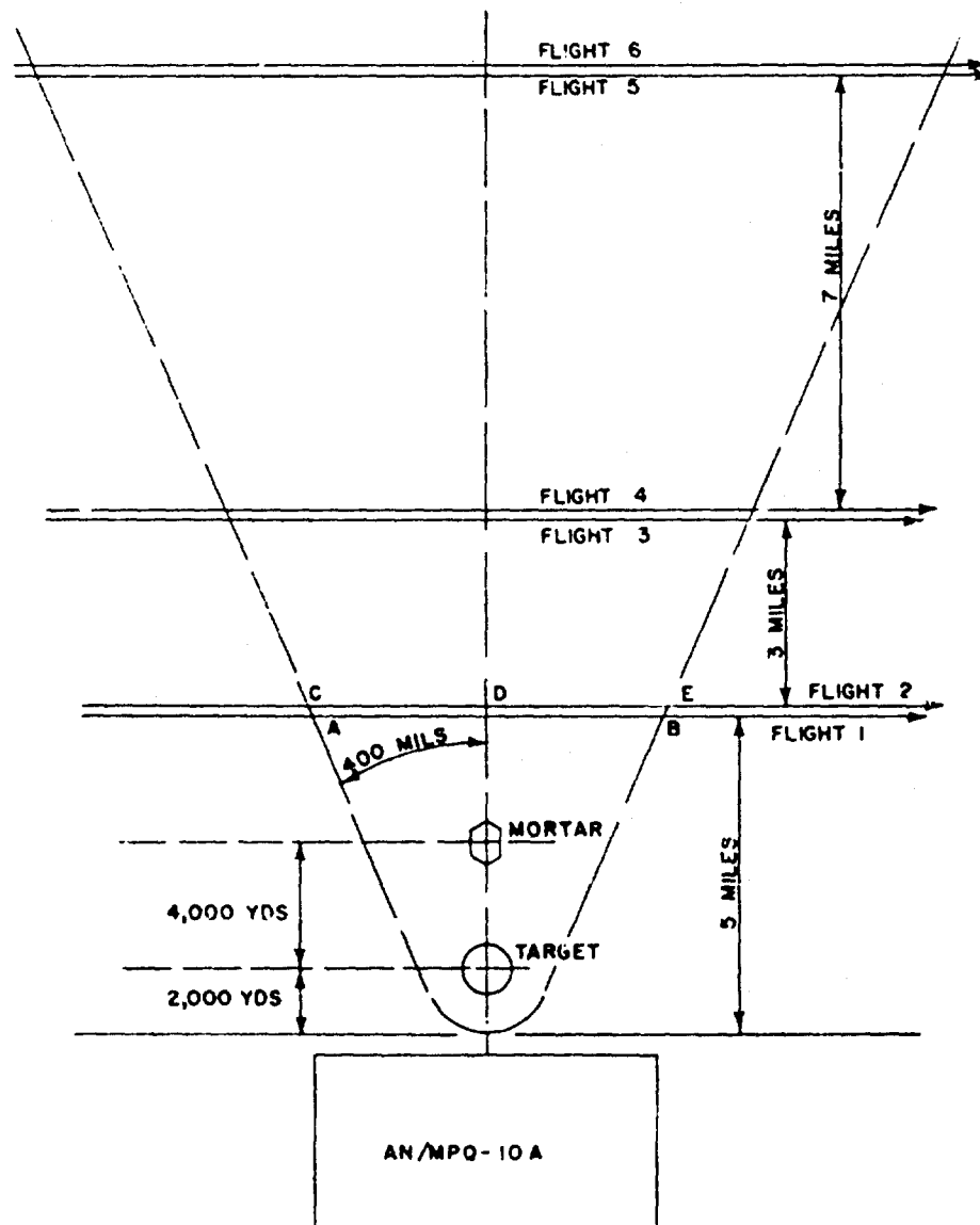
Fig. 10. (CMHA) Flight and location plan for test 11
