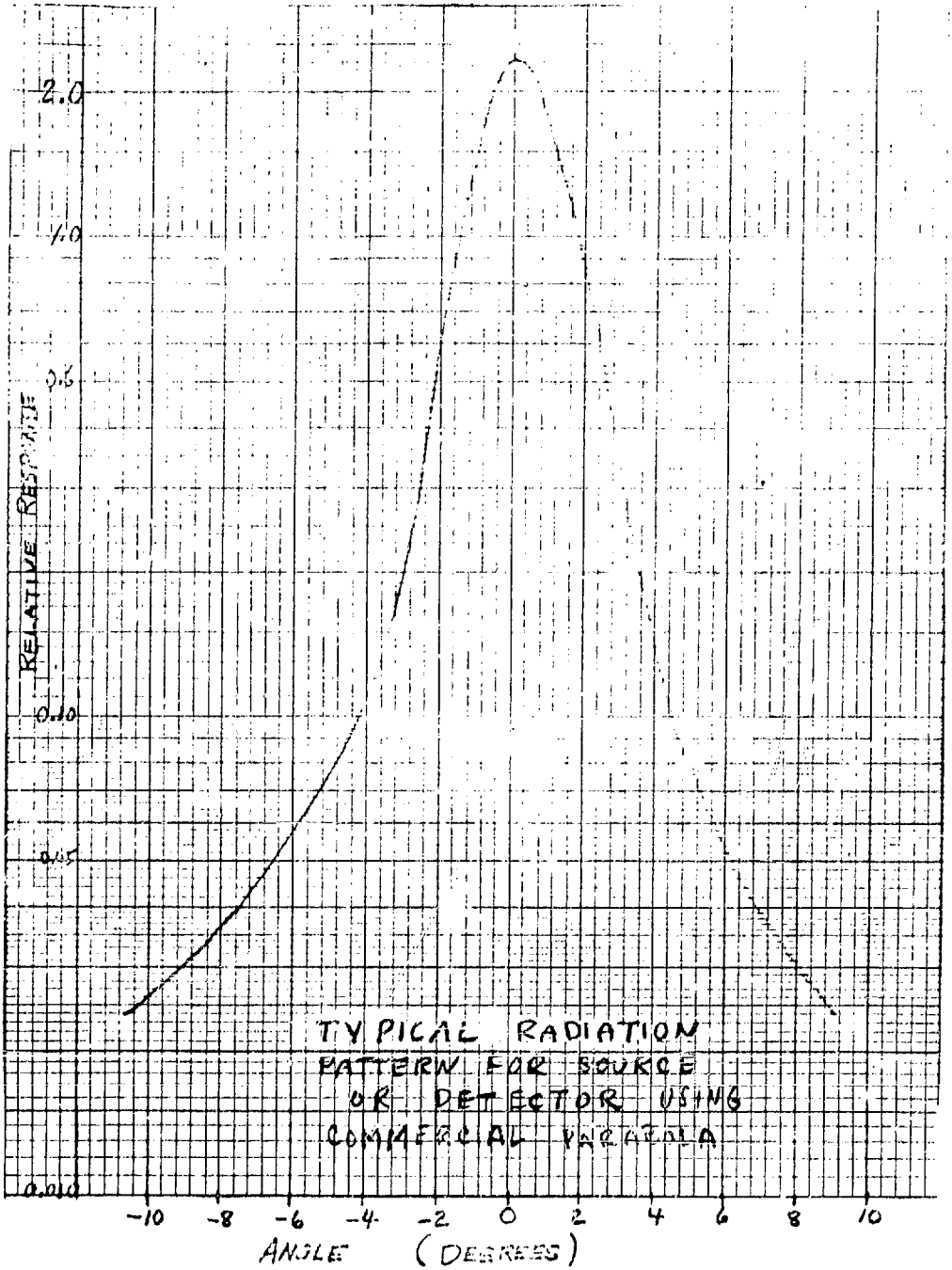
Figure 6. Typical Radiation Pattern for Source or Detector.
