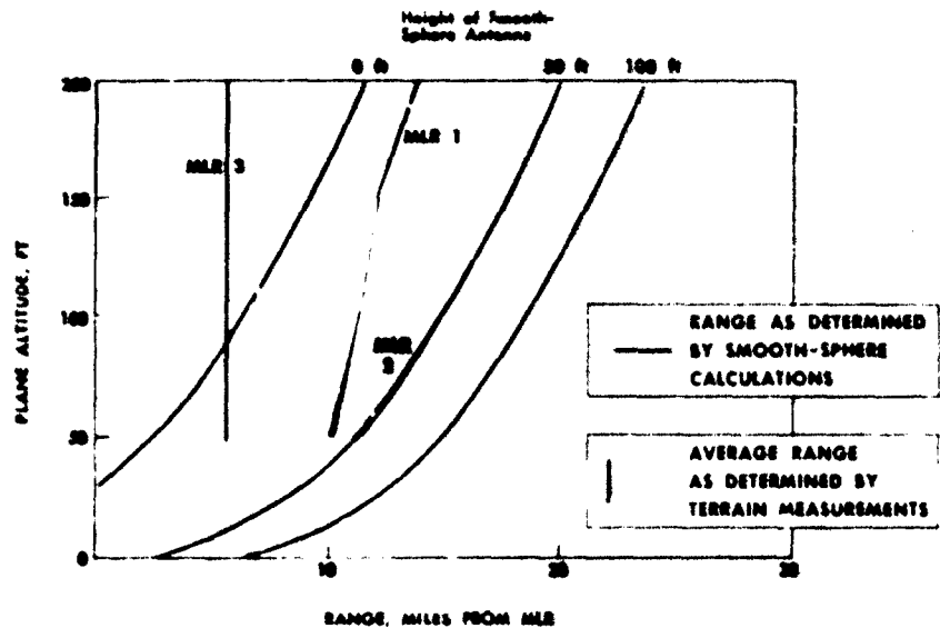
Fig 10 - As this graph shows, theoretical analysis suggests that radar antennae be elevated because, by smooth-sphere calculations, the higher the antennae, the greater the range of detection. But notice that when terrain is taken into account along the MLRs studied, antenna height makes little or no difference. In the case of MLR 3, high ridges make the range practically independent of altitude.
