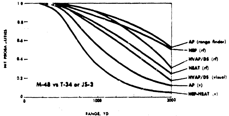
Fig. 14.—This graph shows how the probability of hitting a Soviet tank is affected by the type of projectile used.
