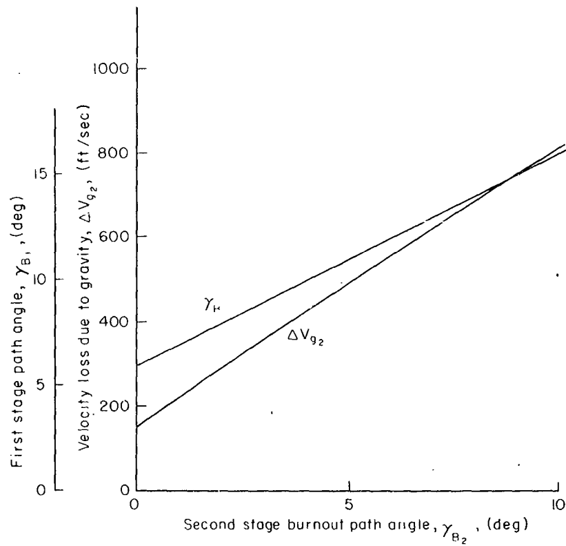
Fig E-2—Velocity loss during second stage
