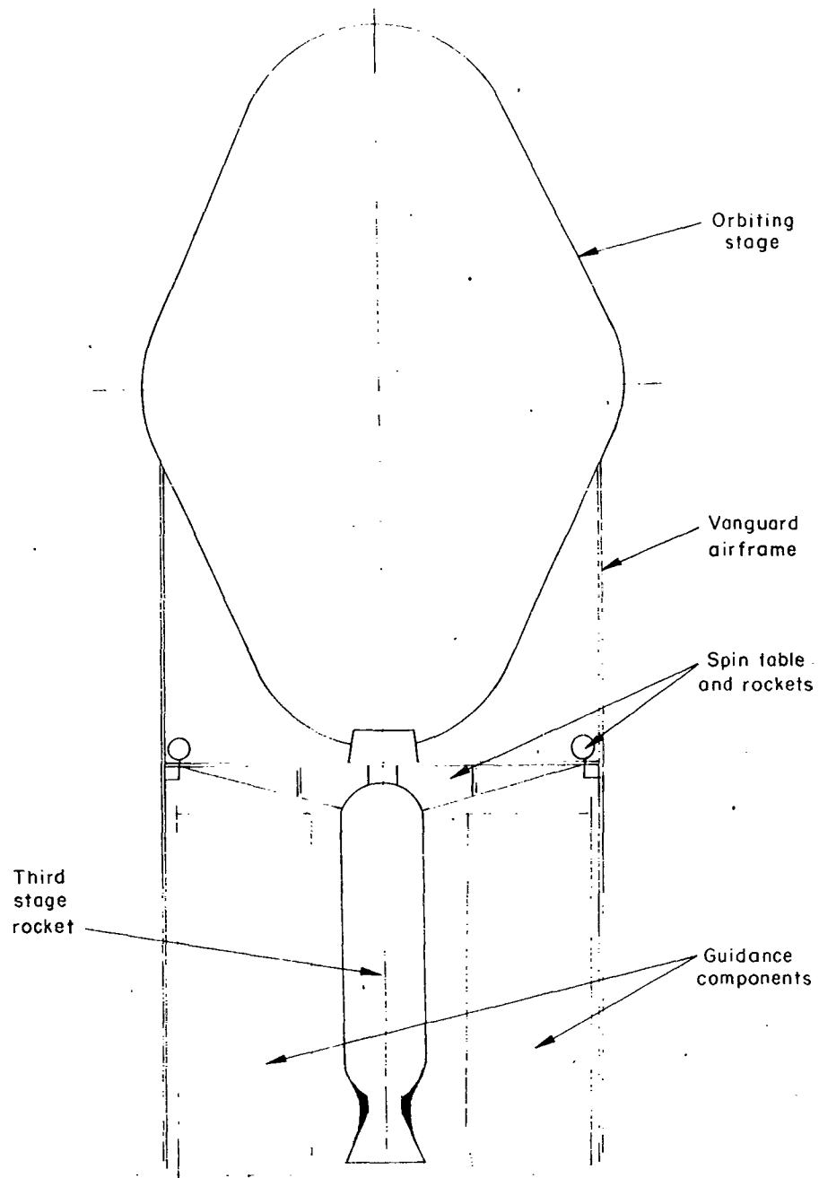
Fig. F-2 — Satellite and third stage rocket
