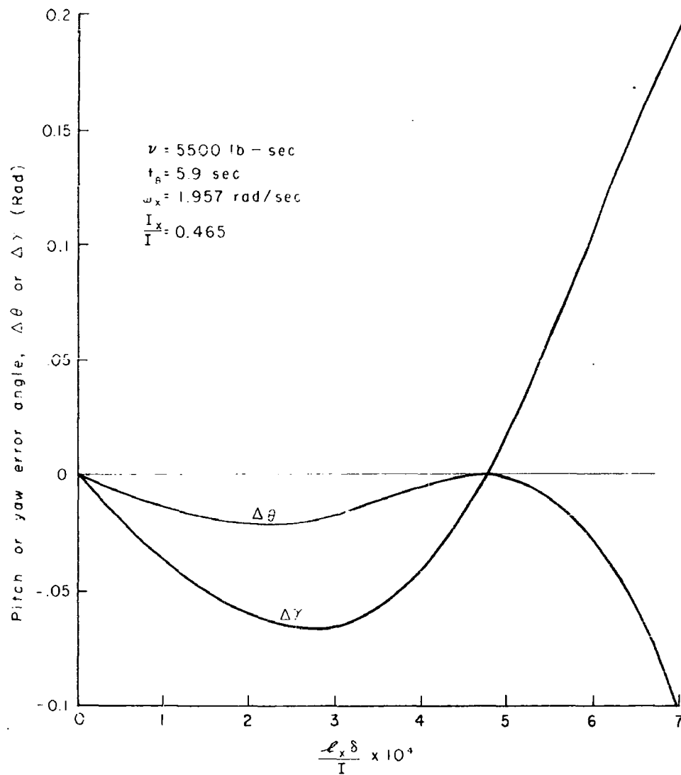
Fig. C-5—Pitch and yaw error angles at the end of burning as a function of the thrust misalignment errors
