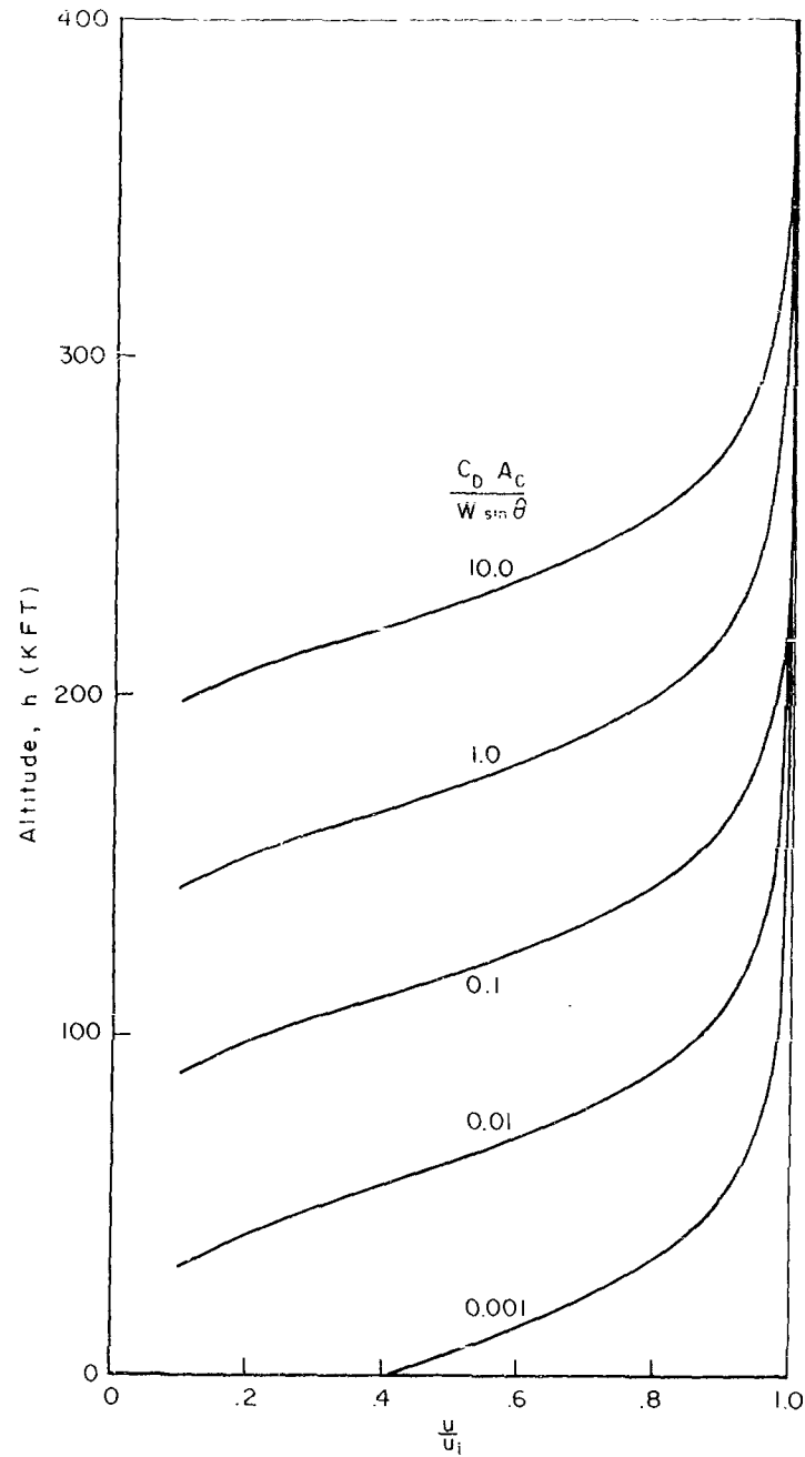
Fig.H-4—Velocity variation with altitude for atmospheric entry
