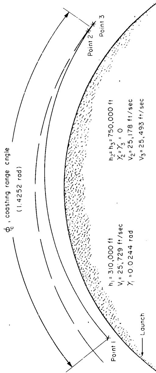
Fig. D-2 — Representative ascent trajectory
