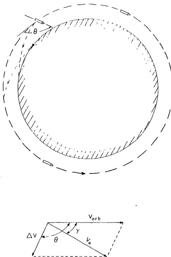
Fig. H-1— Vehicle orientation in orbit and at time of velocity increment
