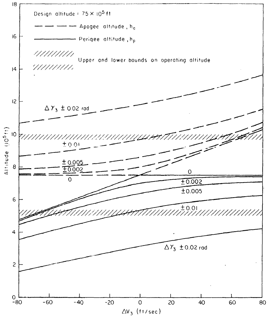
Fig. D-1—Apogee and perigee altitudes related to errors in the magnitude ( \Delta V_3 ) and direction ( \Delta\gamma_3 ) of final burnout velocity.
