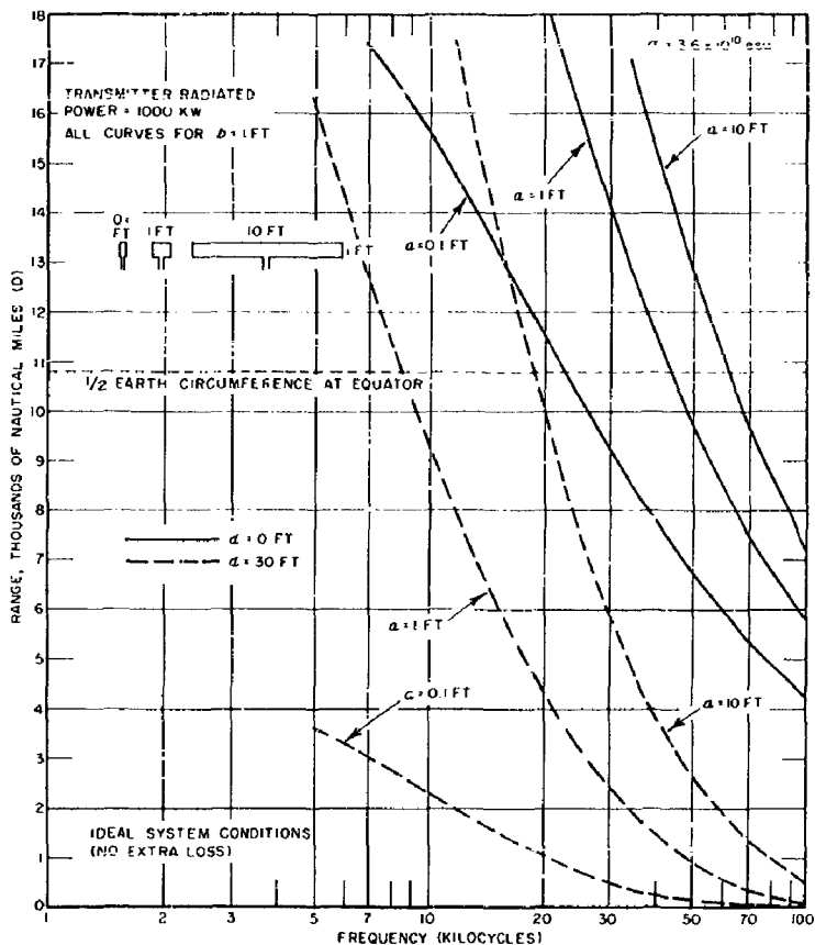
Fig. 20 - Range obtainable based on propagation entirely over sea water with receiving systems having different loop horizontal dimensions and a fixed 2390\text{-}\mu\text{v} design threshold voltage sensitivity. 2390\text{ }\mu\text{v} \approx 2.2\text{ }\mu\text{v/m} at 18.6\text{ kc} with no extra system losses.
