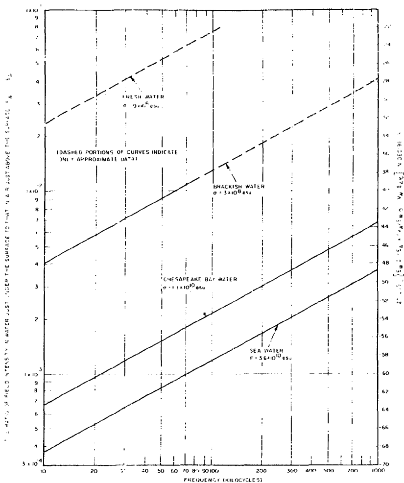
Fig. 4 - Radio electric-field interface transition loss. E_H(0)/E_E \approx \sqrt{f/2\sigma} , where f is frequency in cps and \sigma is conductivity in esu (accurate where \sigma/f \geq 3600 ).
