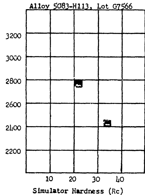
Figure 6. Plate Protection Ballistic Limit vs 20 mm Fragment Simulator Hardness for 1 1/4 inch Aluminum-Magnesium Alloys at 45° Obliquity
