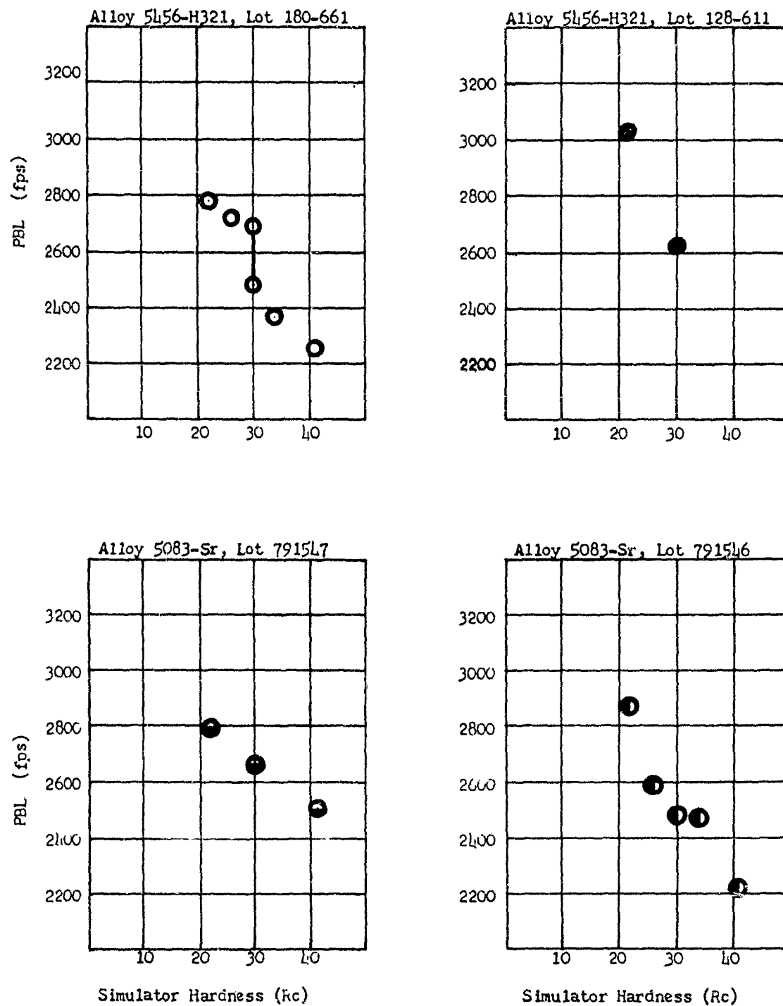
Figure 4. Plate Protection Ballistic Limit vs 20 mm Fragment Simulator Hardness for 1 1/4 inch Aluminum-Magnesium Alloys at 45° Obliquity
