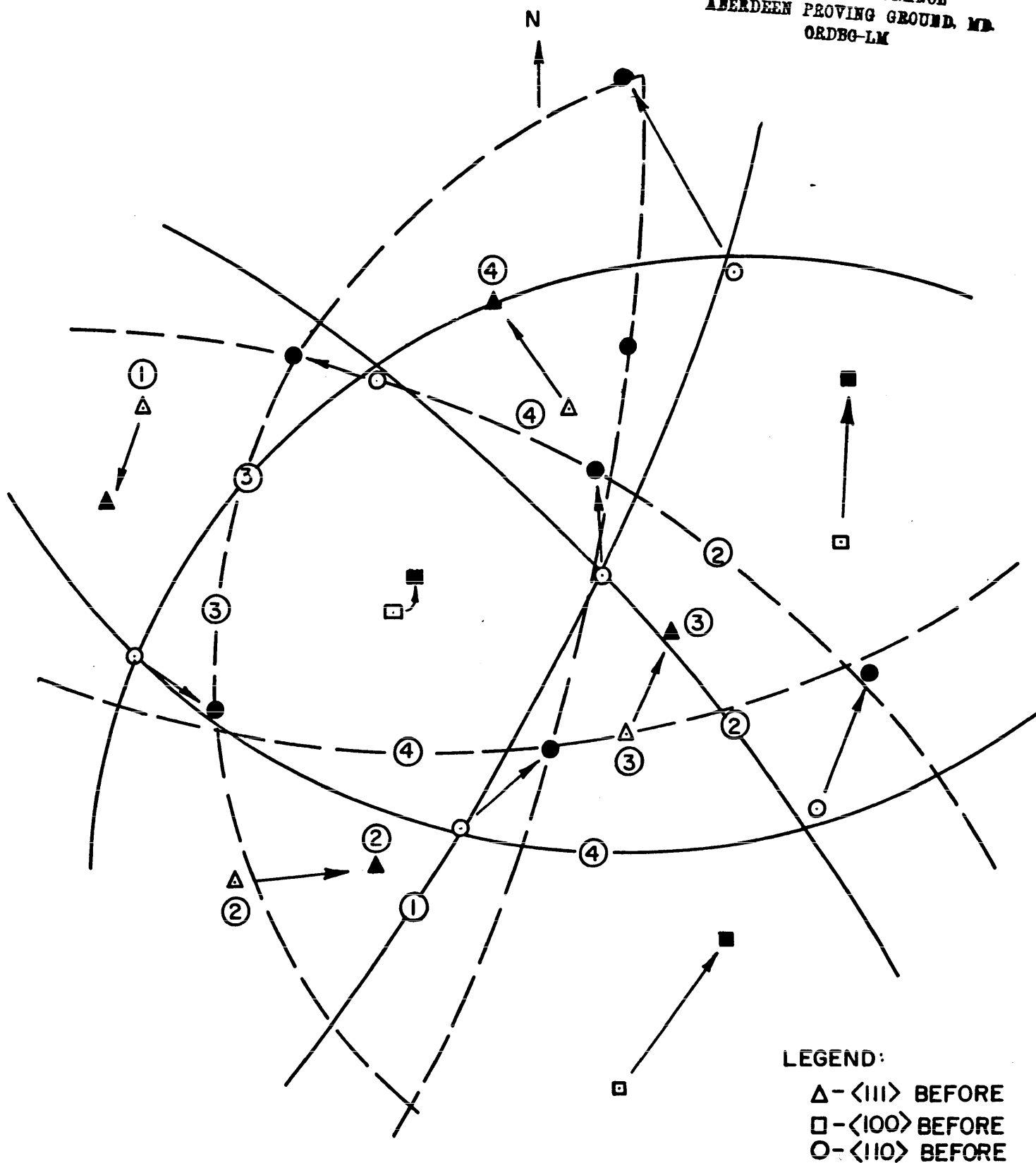
FIG. 28 - STEREOGRAPHIC PLOT OF \langle 100 \rangle \langle 110 \rangle AND \langle 111 \rangle TYPE POLES, BEFORE AND AFTER DEFORMATION
