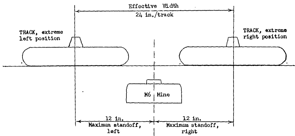
Figure 9 (C): Determination of Lethal Widths for Charge Weights of 24 Pounds or Less.
