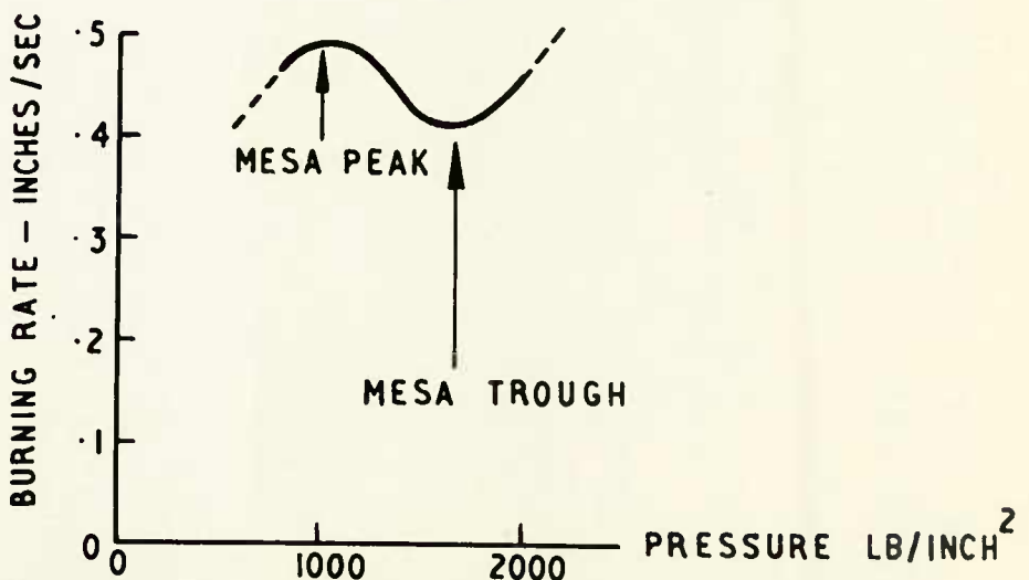
FIG. 1 (e) TYPICAL BURNING RATE CURVE FOR 'MESONIC' PROPELLANT
