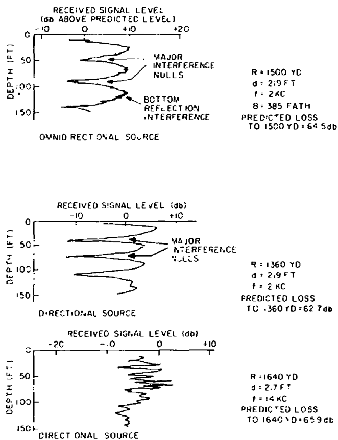
Fig. 5 - Received signal vs depth profiles (experimental)
