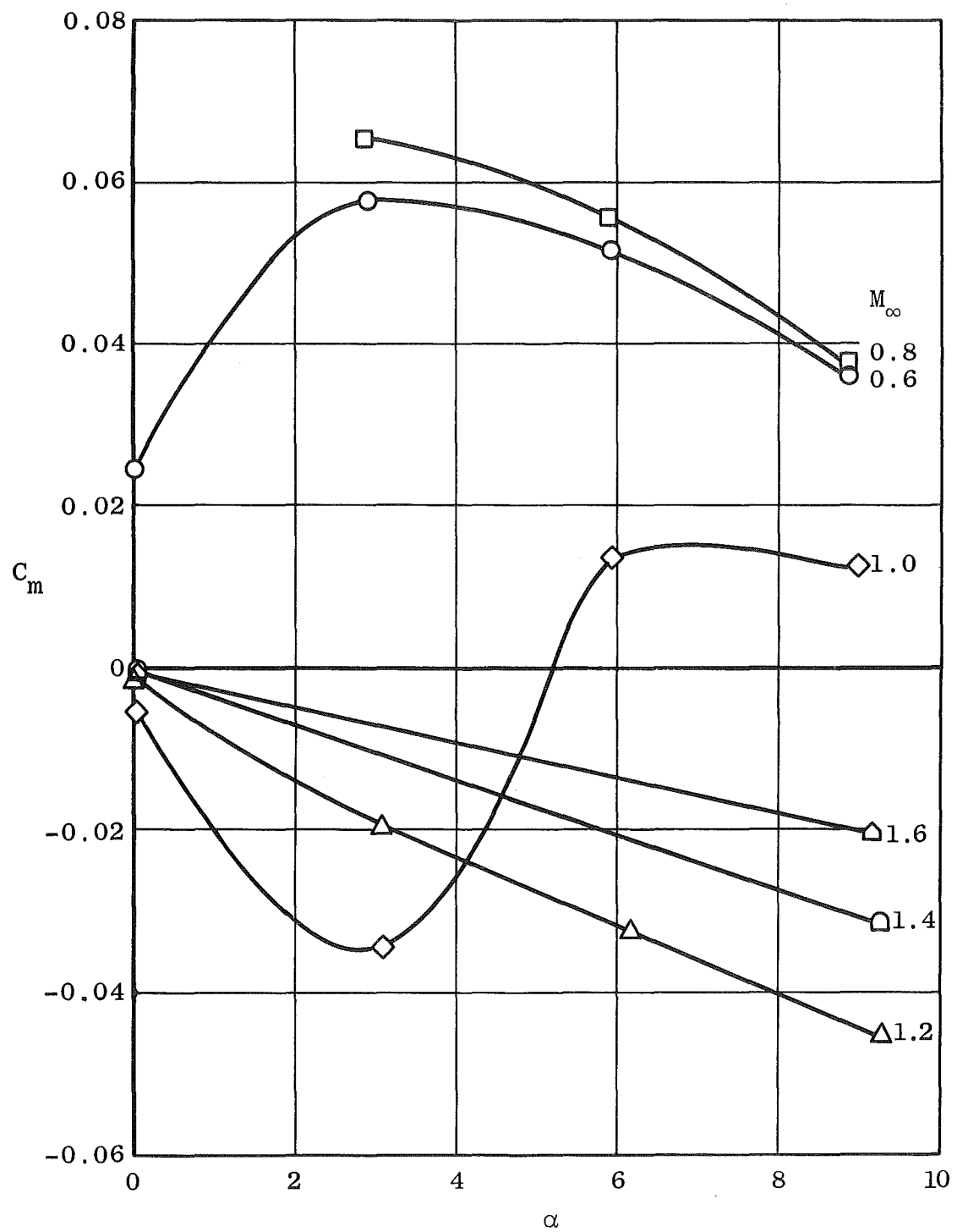
Fig. 13 Effect of Angle of Attack and Mach Number on Pitching-Moment Coefficient, \psi = 180
