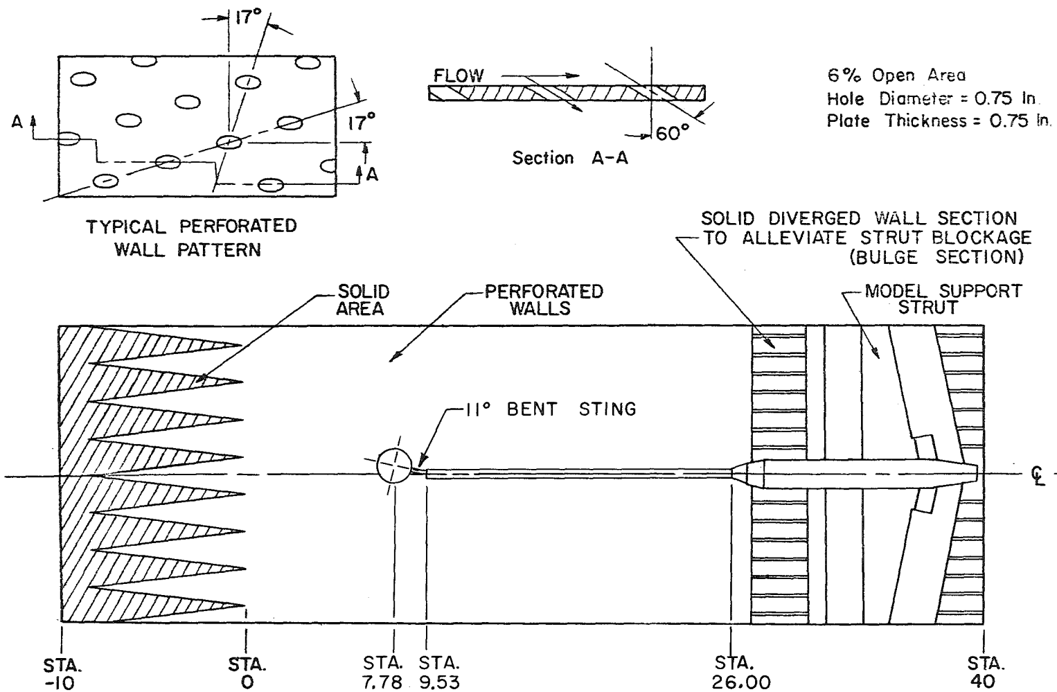
Fig. 1 Model Installation and Details of the Perforated Walls
