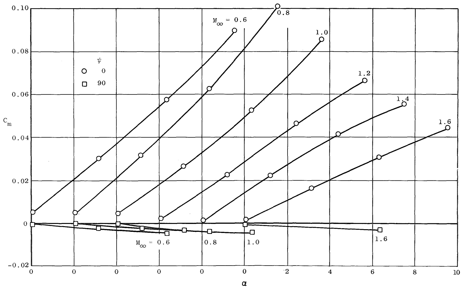
Fig. 12 Effect of Angle of Attack and Mach Number on Pitching-Moment Coefficient, \psi = 0 and 90
