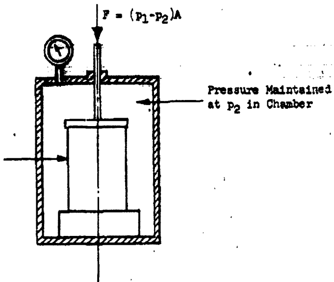
FIGURE 4.1.4 TRIAXIAL TEST FIXTURE
