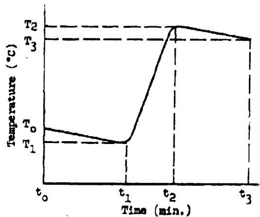
a) Calorimeter Above Room Temperature
