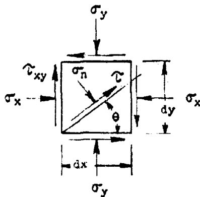
FIGURE 4.1.2 RESOLUTION OF STRESSES
