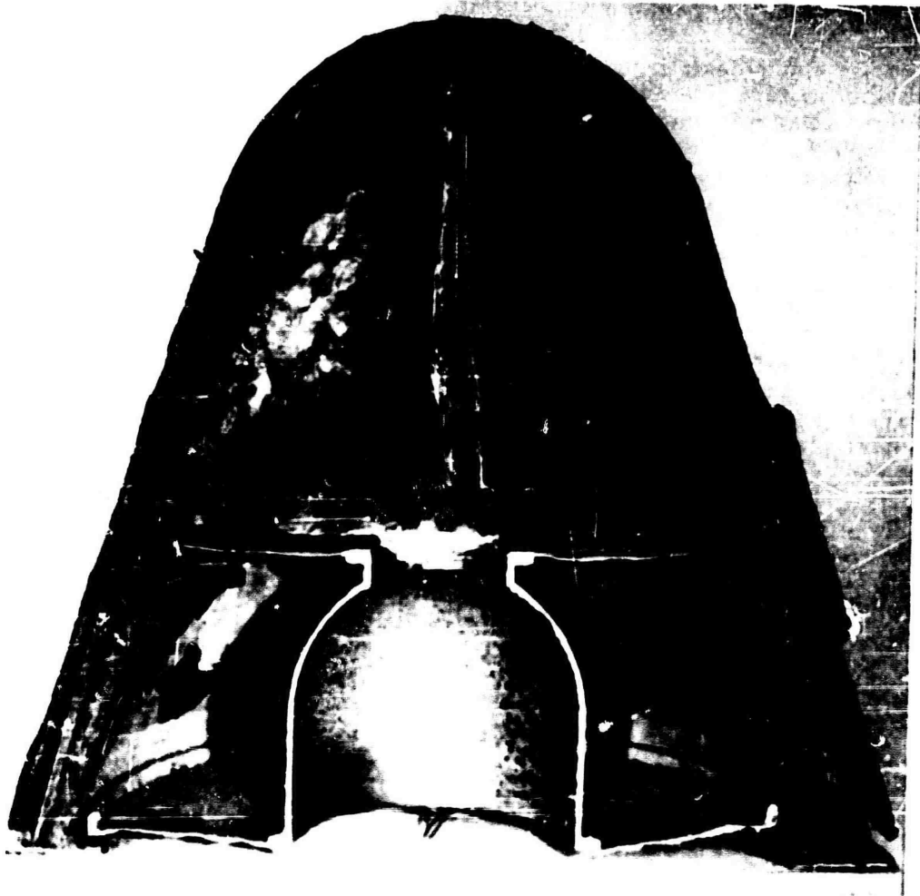
FIG. 22. Nose Cone, Sectioned After Test.
