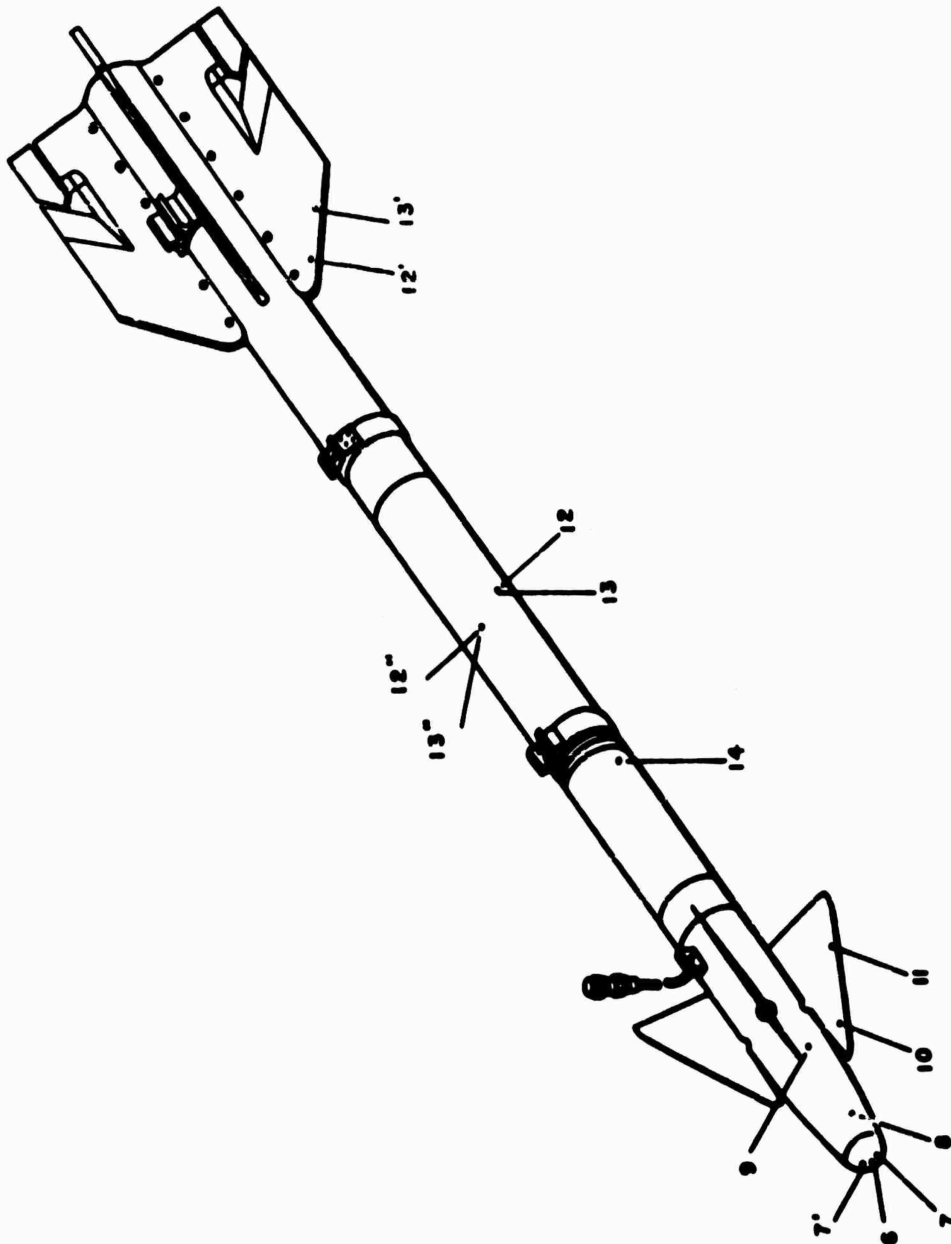
FIG. 7. Thermocouple Channel Numbers for the Temperature-Telemetering Round.
