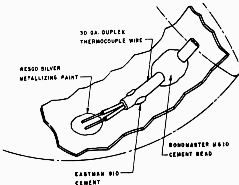
FIG. 3. Dome Thermocouple Installation.
