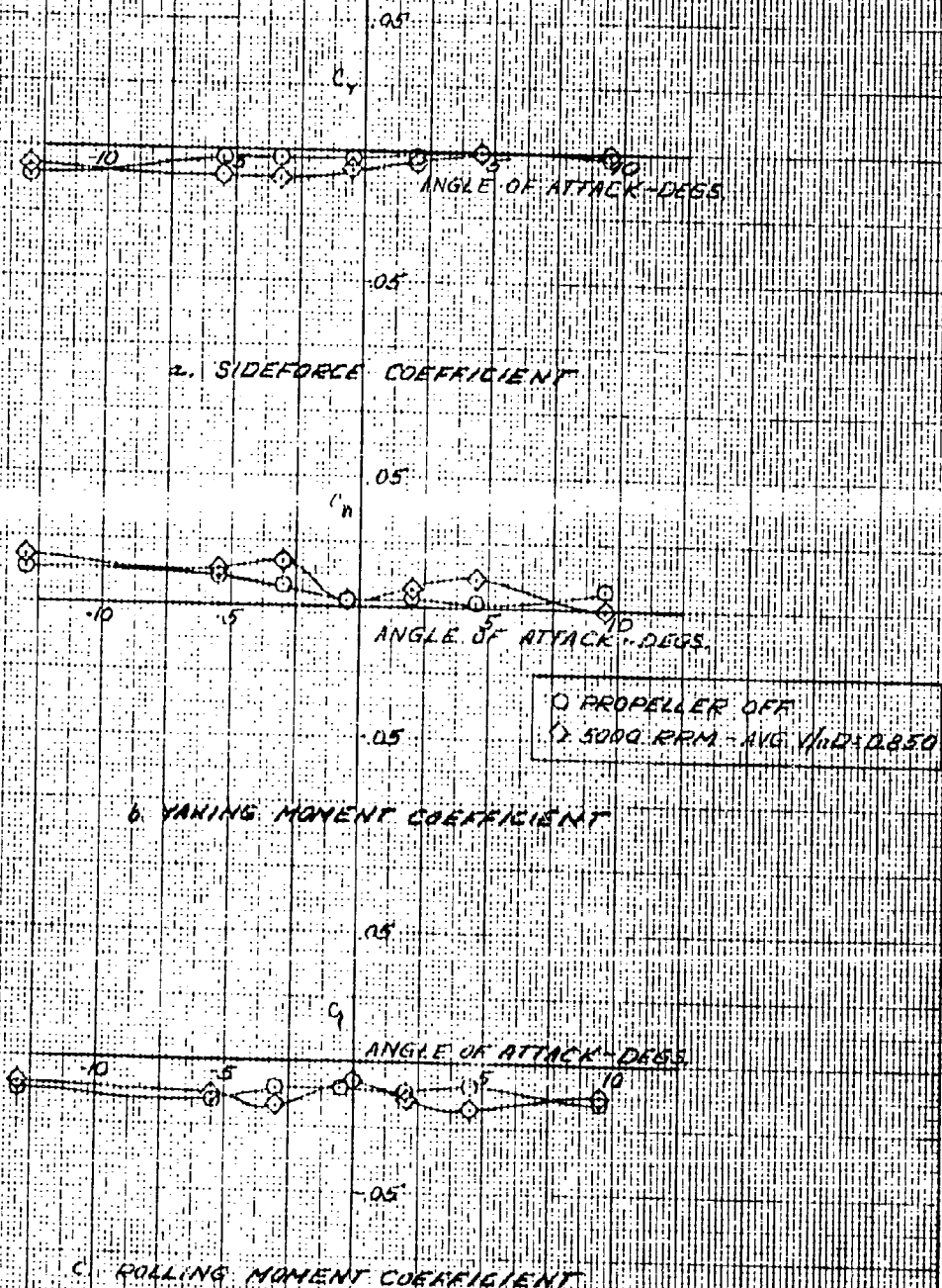
FIGURE 4.5 TYPICAL EFFECT OF WAKE PROPELLER ON THE LATERAL AERODYNAMIC CHARACTERISTICS IN PITCH (CROSS-COEFFICIENTS) GAC PROPELLER - \beta = 20^\circ V_0 = 141 TO 144 FT/SEC (ELTP)
