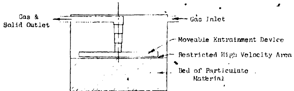
FIGURE 8. PNEUMATIC FEEDING SYSTEM IN WHICH THE SOLIDS ARE ENTRAINMENT FROM A FREE SURFACE BY A HIGH VELOCITY GAS STREAM.
