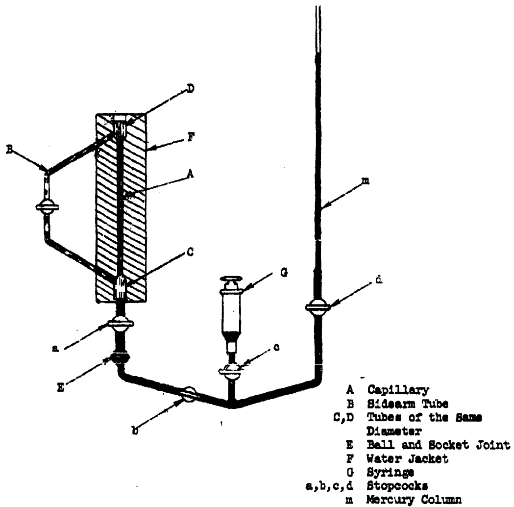
FIGURE 5.2.3 CAPILLARY VISCOMETER
