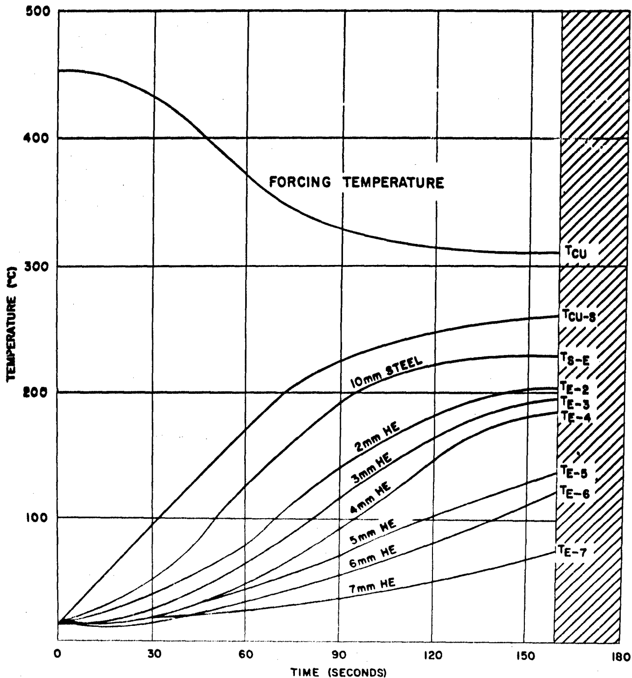
FIG. 3 DEFLAGRATION OF TNT. INITIAL FORCING TEMPERATURE, 456°C.
