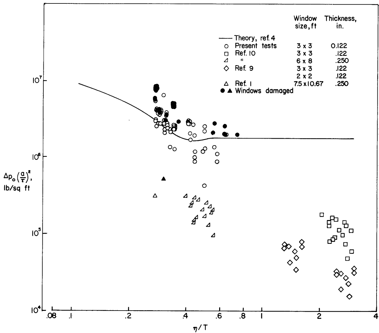
Figure 27.- Summary of window-glass breakage experience due to sonic booms.
