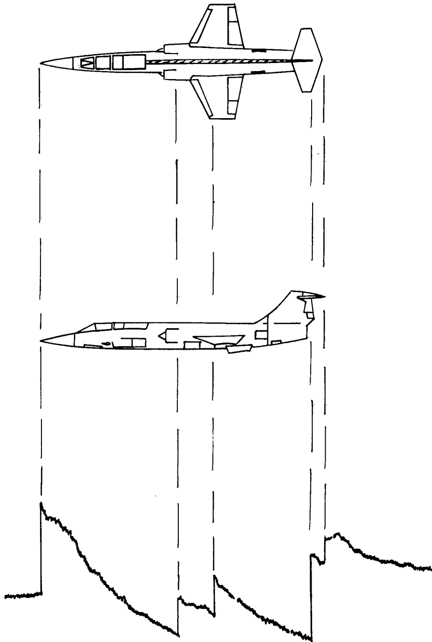
Figure 14.- Planform and side views of airplane A with a typical time history of shock noise pressure.
