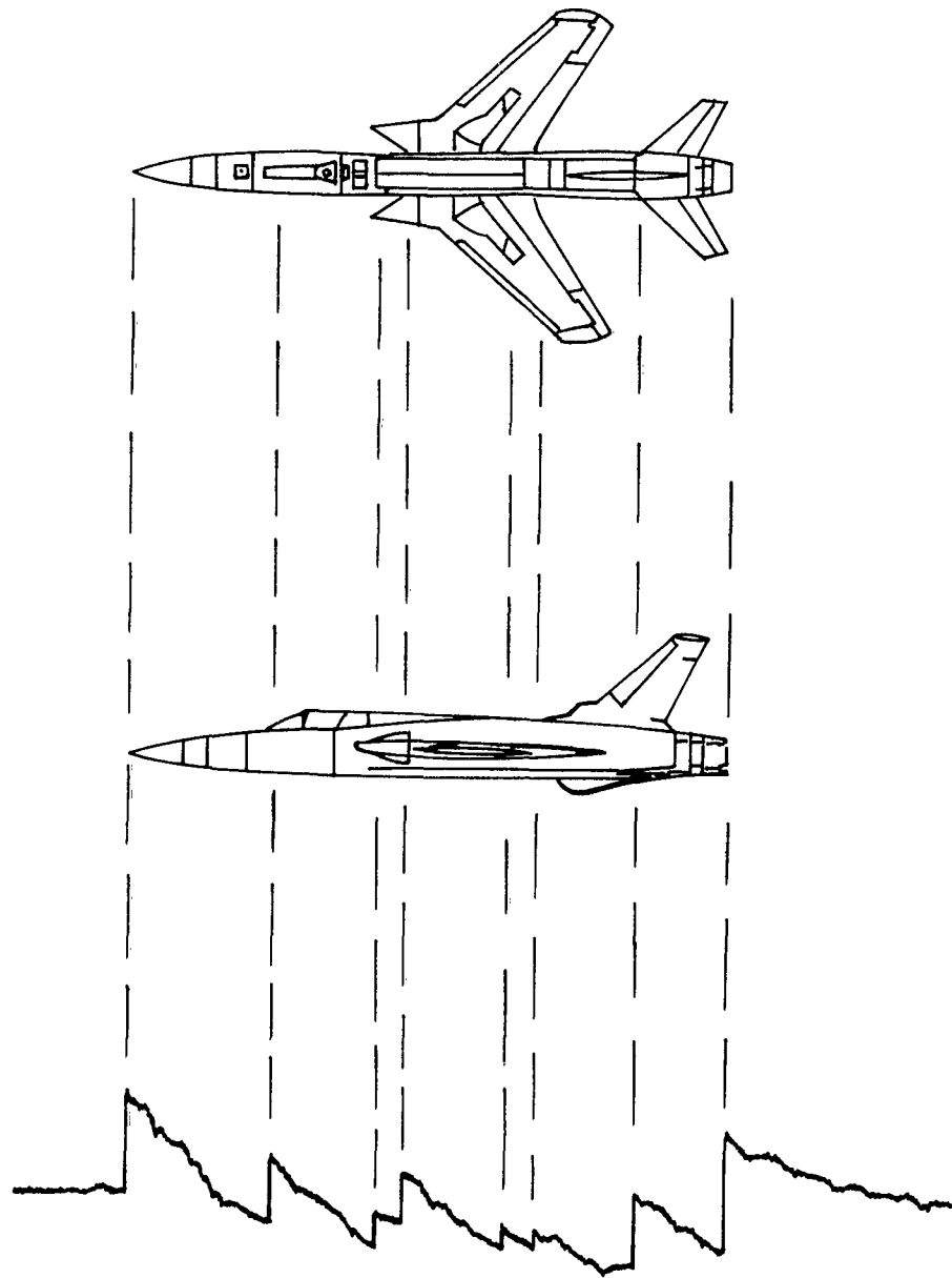
Figure 15.- Planform and side views of airplane B with a typical time history of shock noise pressure.
