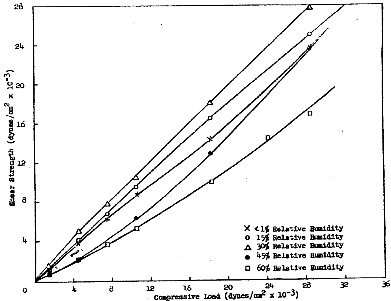
FIGURE 3.2.2 Shear Strength of Sn Powder as a Function of Compressive Load
