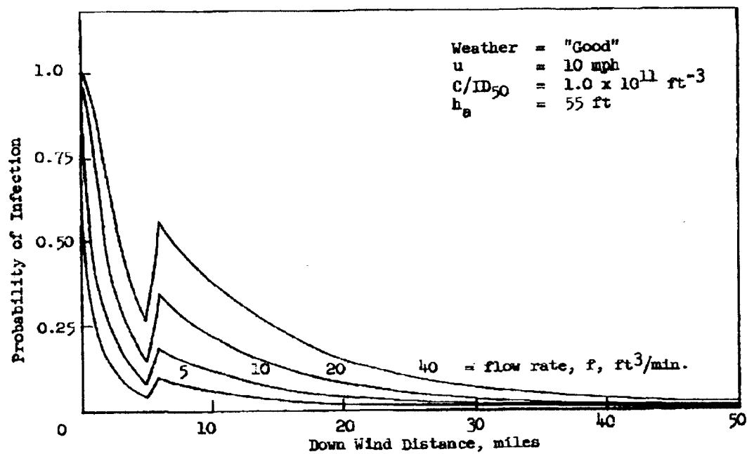
FIGURE 9.5.1 Probability of Infection versus Cloud Travel for C/ID_{50} = 1 \times 10^{11} \text{ ft}^{-3}
