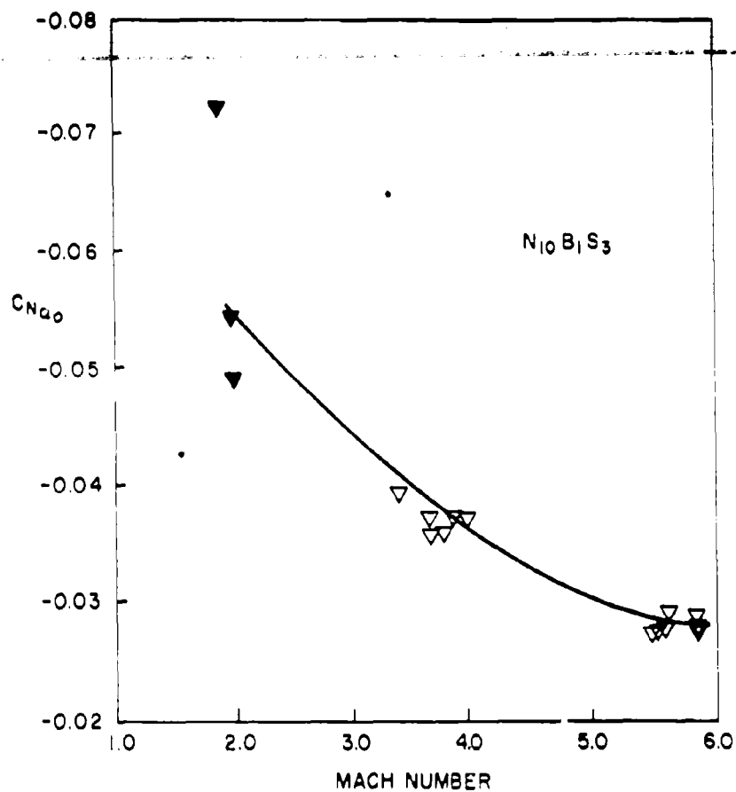
SOLID POINTS NOT CORRECTED TO ZERO YAW FIG. 7C C_{Na_0} VERSUS MACH NUMBER
