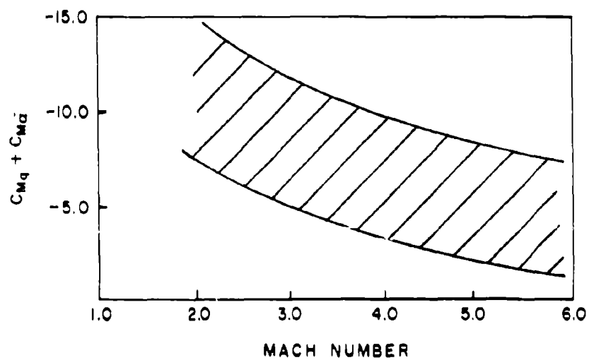
FIG. II C_{Mq} + C_{Ma} VERSUS MACH NUMBER
