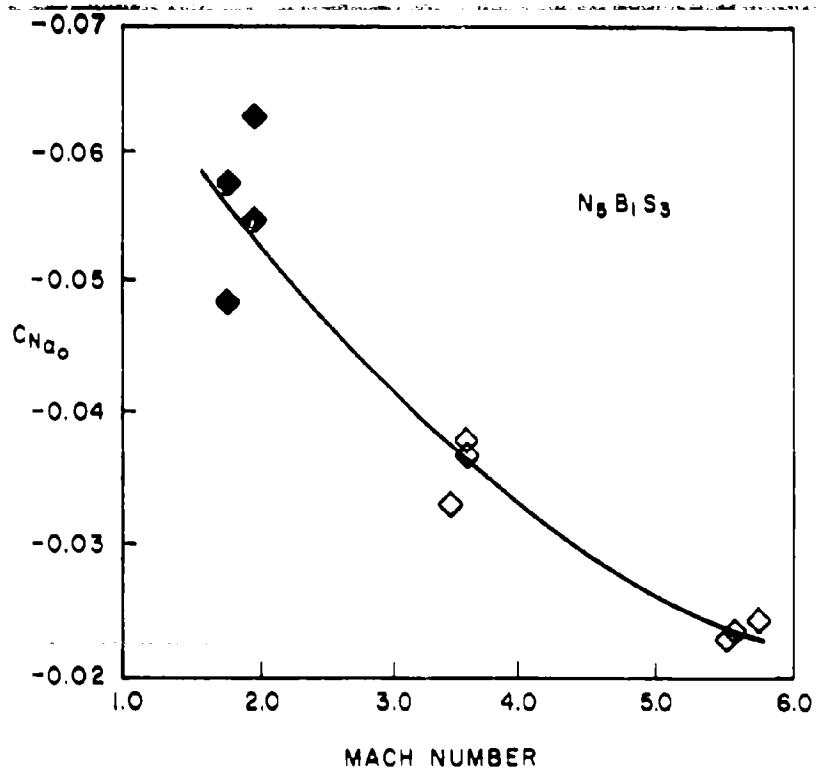
SOLID POINTS NOT CORRECTED TO ZERO YAW FIG.7B C_{N_{a_0}} VERSUS MACH NUMBER
