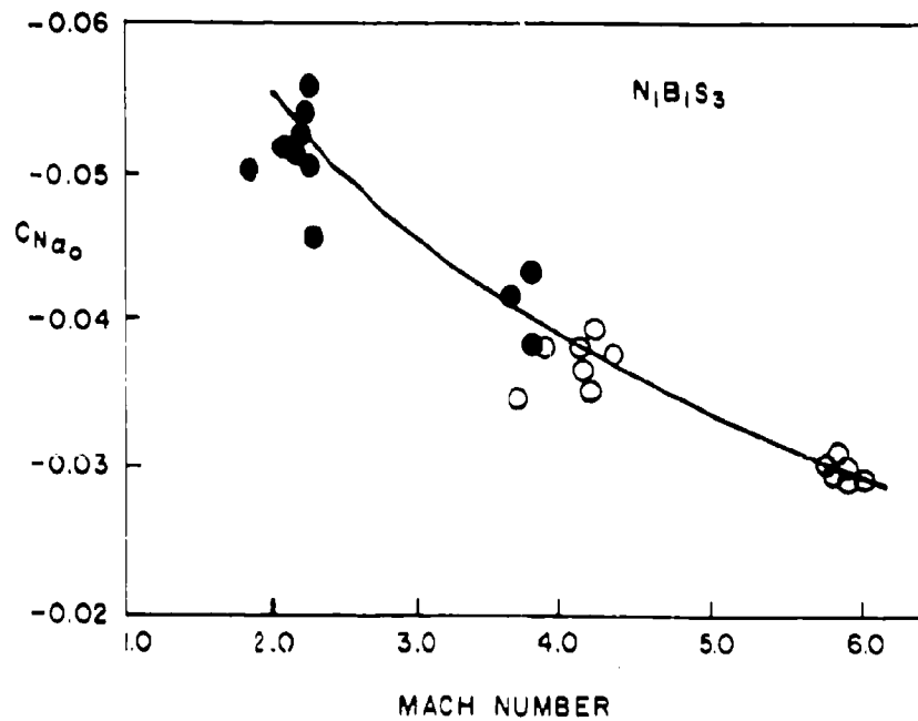
SOLID POINTS NOT CORRECTED TO ZERO YAW FIG. 7A C_{Na_0} VERSUS MACH NUMBER
