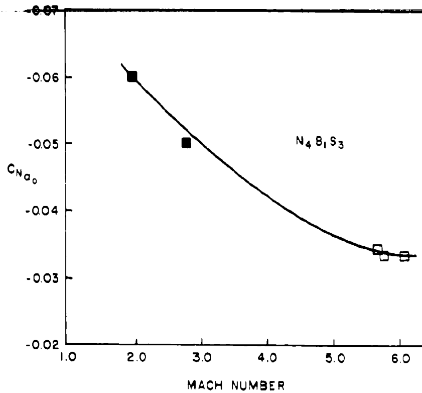
SOLID POINTS NOT CORRECTED TO ZERO YAW FIG.7E C_{Na_0} VERSUS MACH NUMBER
