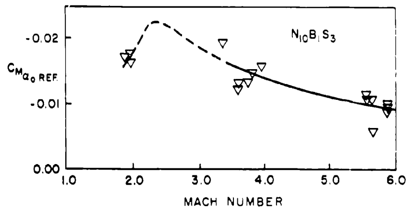
SOLID POINTS NOT CORRECTED TO ZERO YAW FIG. 9A CM_{a_0 REF.} VERSUS MACH NUMBER
