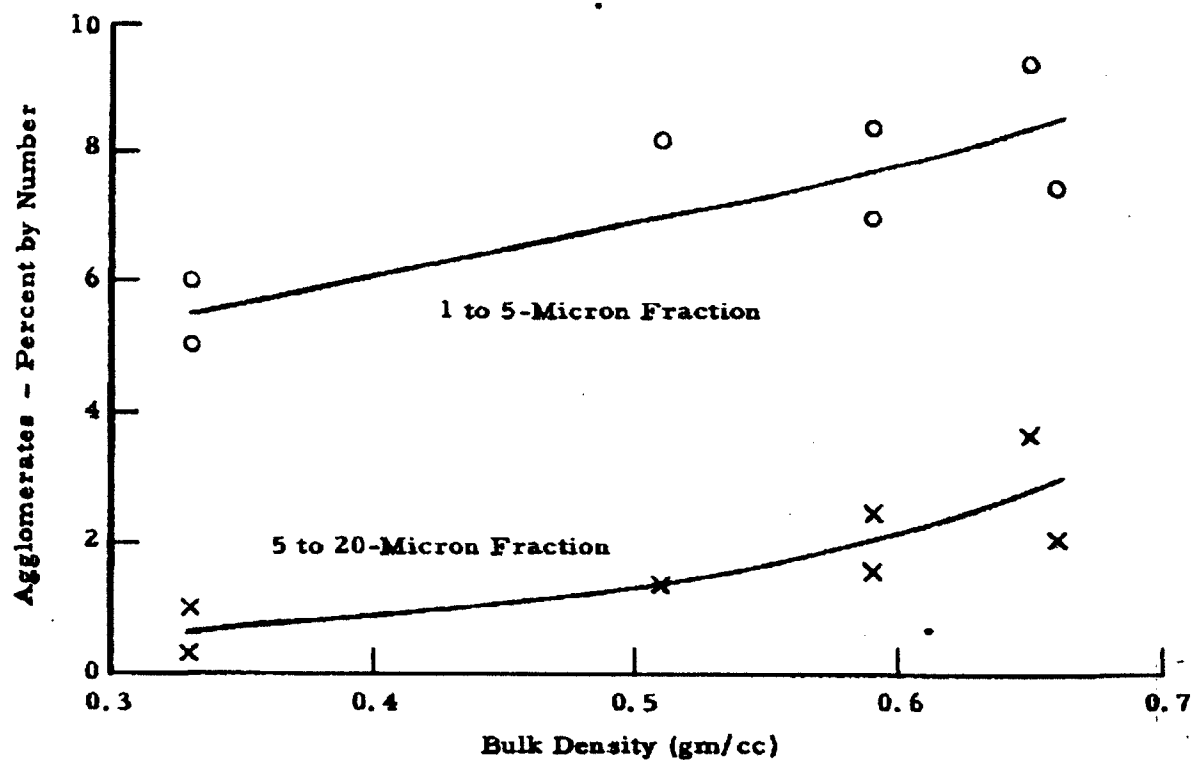
Figure 5.4 Percentage of Sm Aerosol Particles (by number) Consisting of Agglomerates in the 1 to 5-Micron and 5 to 20-Micron Ranges (Wind tunnel Mach number 0.5; sampling position - 0.63 cm below tunnel top wall)
