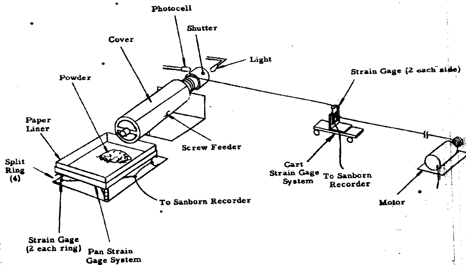
Figure 3.13 Experimental Set-Up for Torque and Output Measurements of Screw Feeder
