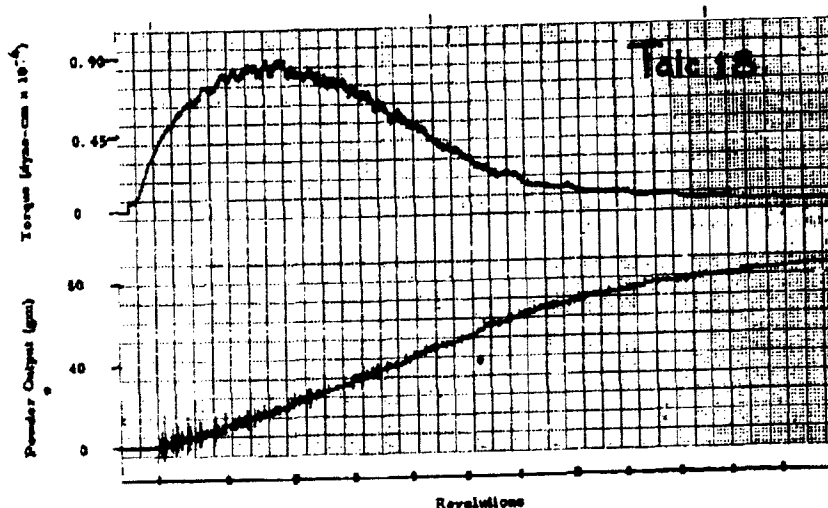
Figure 3.14 Screw Feeder Torque and Output Data for Cornstarch, Polyvinyl Alcohol and Talc Powder
