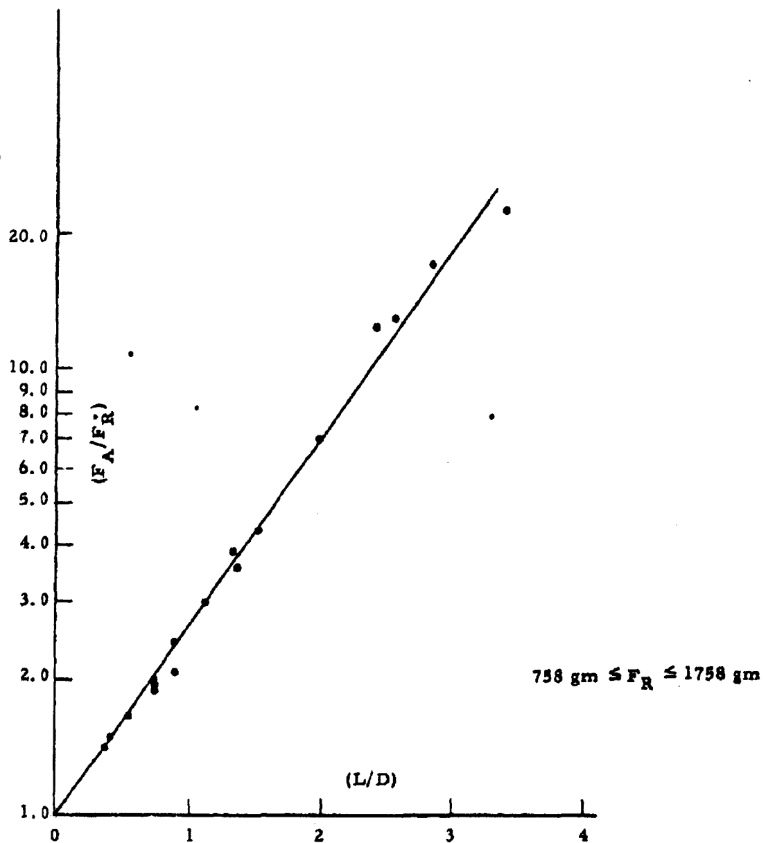
Figure 3.11 Piston-Cylinder Results on B g (Uncompacted)
