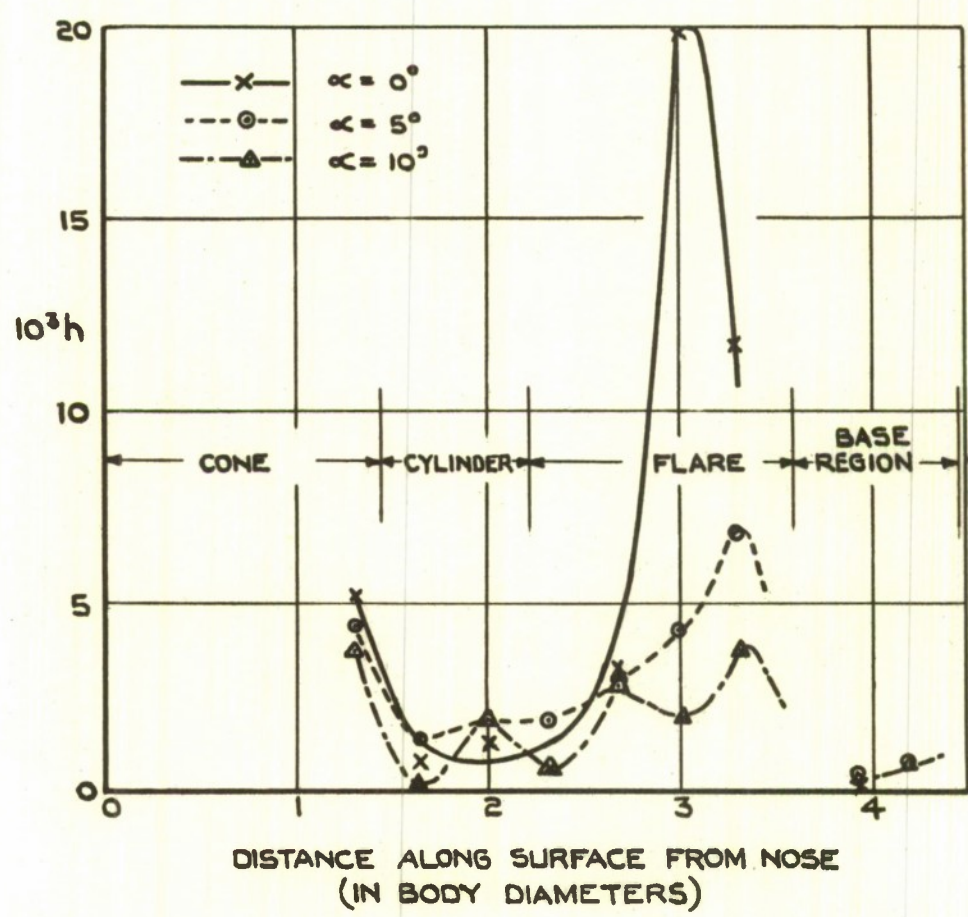
FIG.6. VARIATION OF HEAT TRANSFER FACTOR ALONG MODEL.
