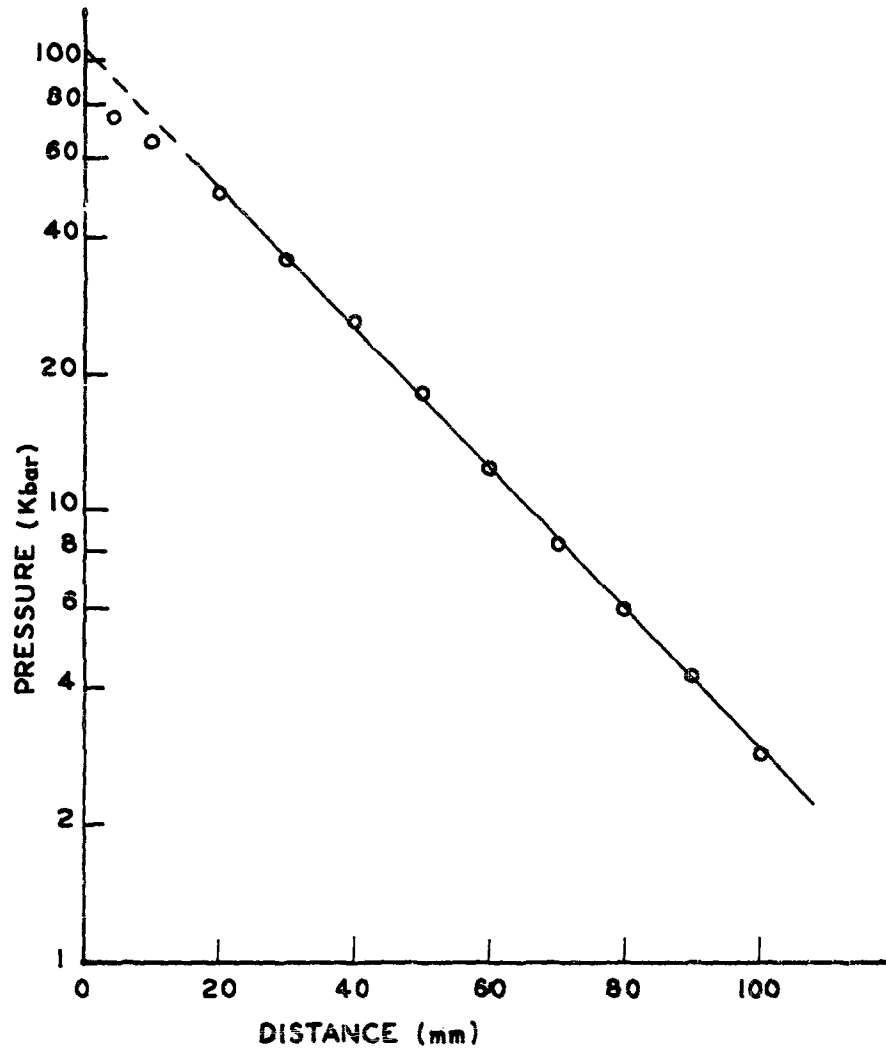
FIGURE 4. Log of Pressure versus Distance in Lucite, loaded as in gap test.
