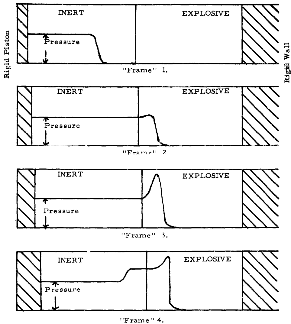
FIGURE 7. One Dimensional Theoretical Model for Gap Test. Inert Gap and explosive have the same equation of state. Progress of shock as a function of time. Piston moves at constant Velocity.
