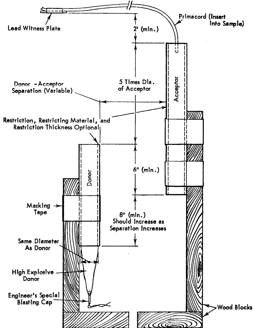
FIGURE 3 Small-Scale Shock and Fragment Impact Test Assembly
