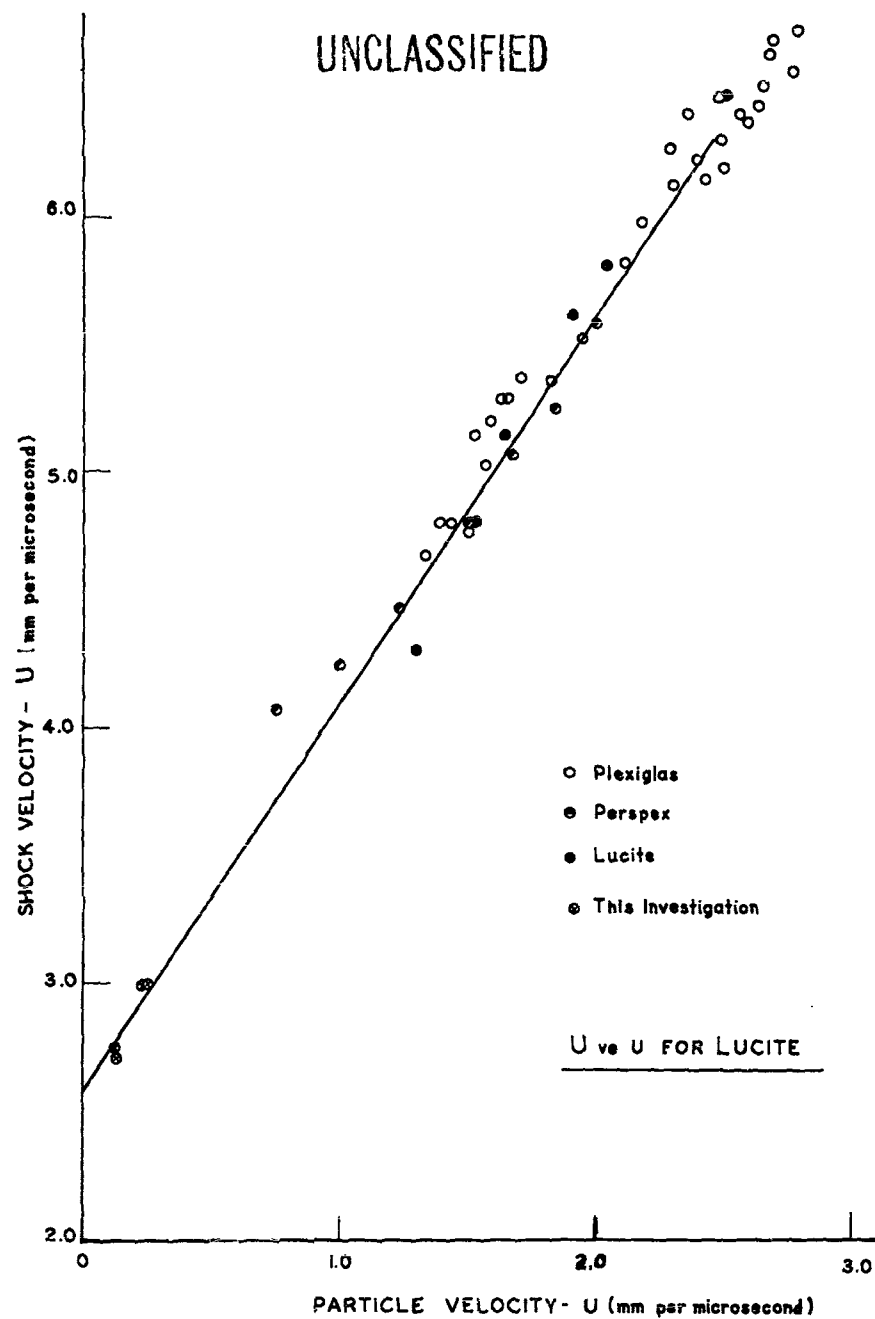
FIGURE 2. Shock versus Particle Velocity in Lucite
