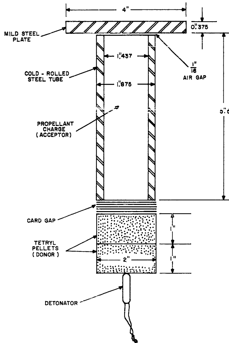
FIGURE 1. Gap Test for Solid Propellants
