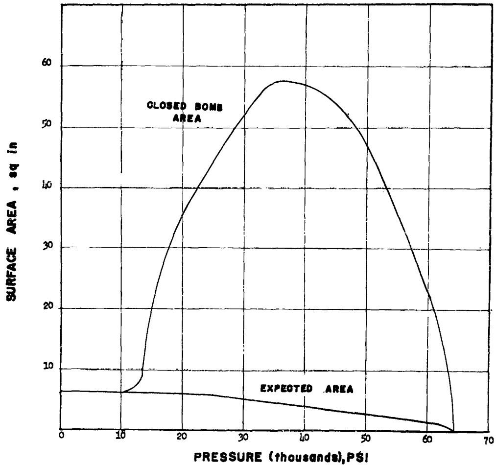
EXPECTED SURFACE AREA VS ACTUAL AREA OBTAINED FOR COMPOSITION B CYLINDER BURNED IN CLOSED BOMB
