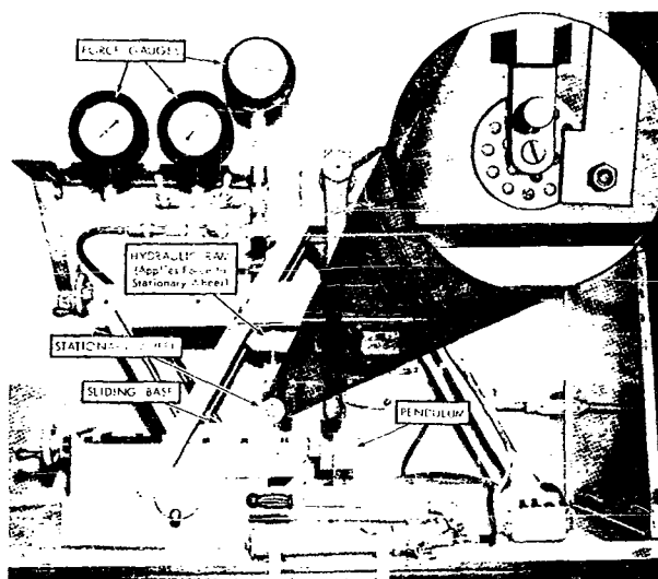
"B" - ABL Sliding Friction Machine
