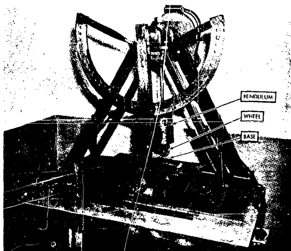
"A" - ABL Pendulum Friction Machine
