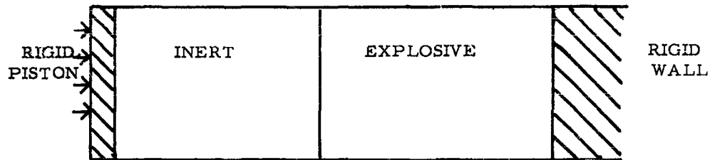
FIGURE 6. One Dimensional Model For Theoretical Treatment of Gap Test. Rigid Piston at Left Compresses Inert Material and Explosive Against Rigid Wall at Right.
