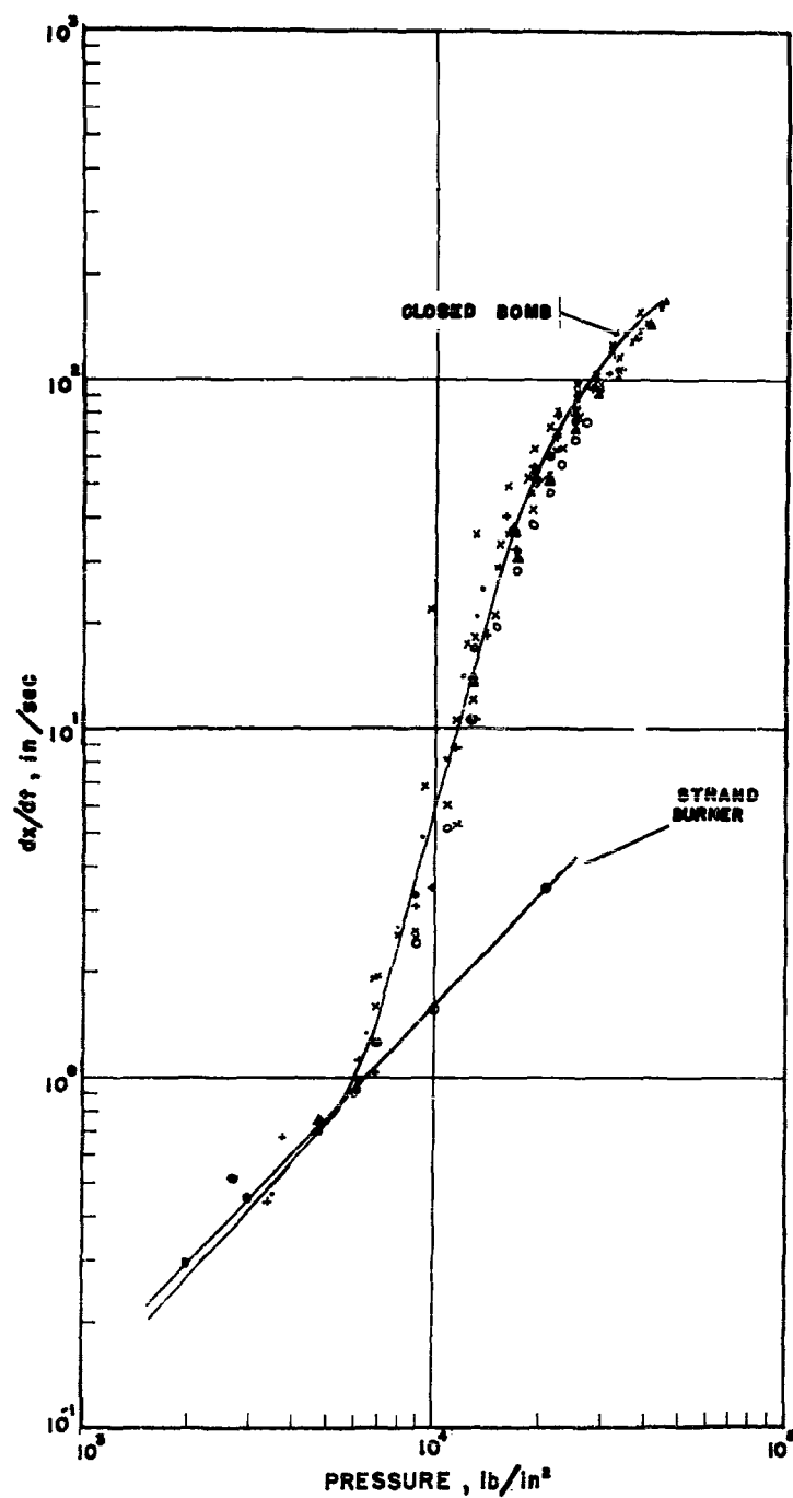
LINEAR BURNING RATES OF TNT OBTAINED WITH CLOSED BOMB AND STRAND BURNER
