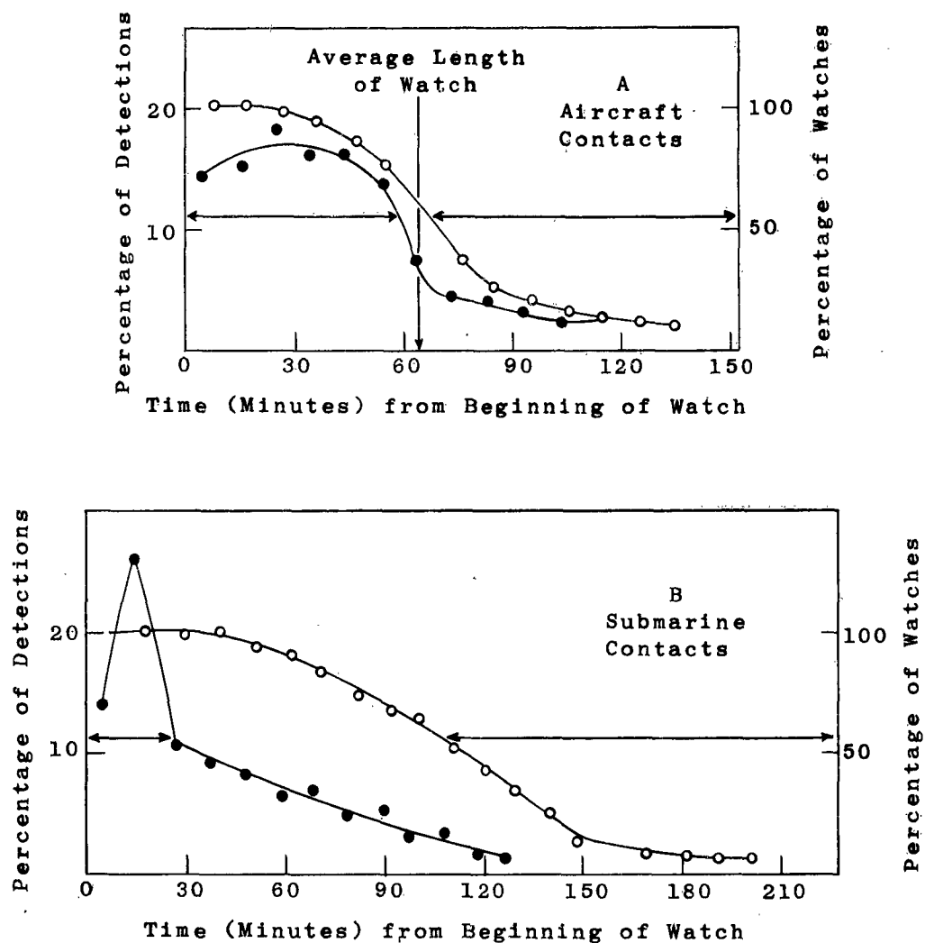
Figure 5. Cumulative percentages of lengths of radar watches (right ordinates) and percentages of aircraft and submarine detections (left ordinates) as a function of time on radar watch.
