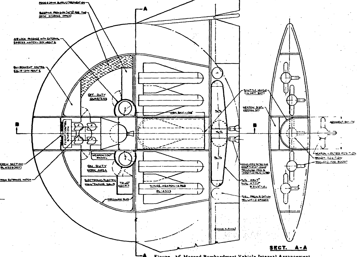
Figure 16. Manned Bombardment Vehicle Internal Arrangement
