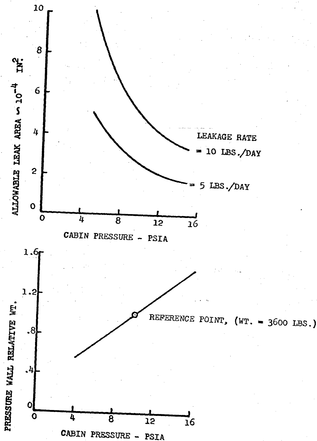
Figure 12. APPROXIMATE EFFECT ON CABIN PRESSURE ON LEAKAGE AND STRUCTURAL WEIGHT
