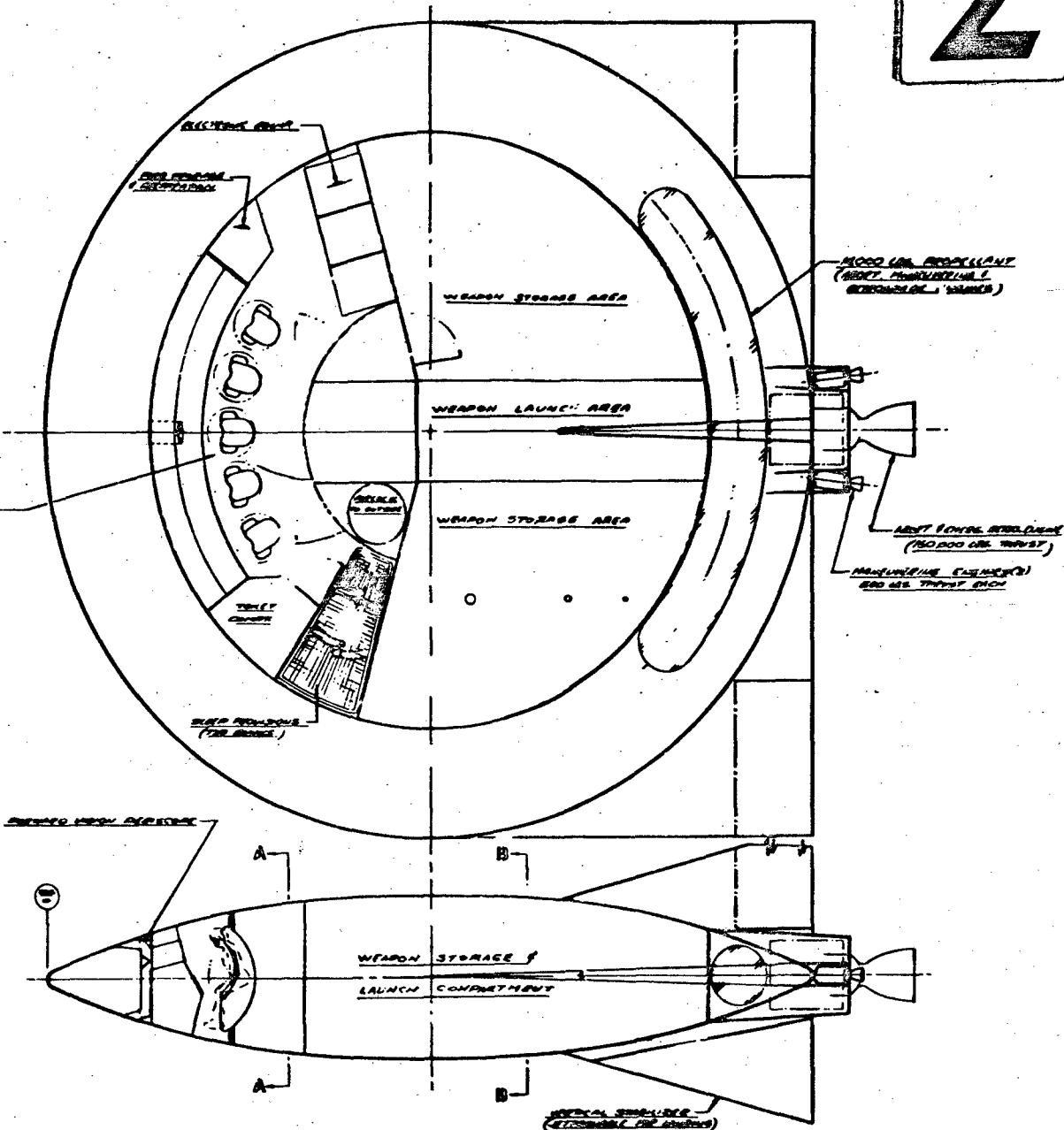
Figure 13 Disc Shape Design Study
