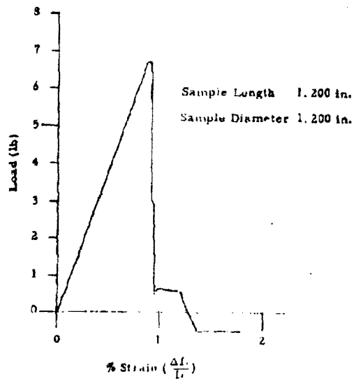
Figure 2.6 Load-Strain Curve for Compacted Saccharin ( \rho_0 = 0.65 \text{ g/cm}^3 )
