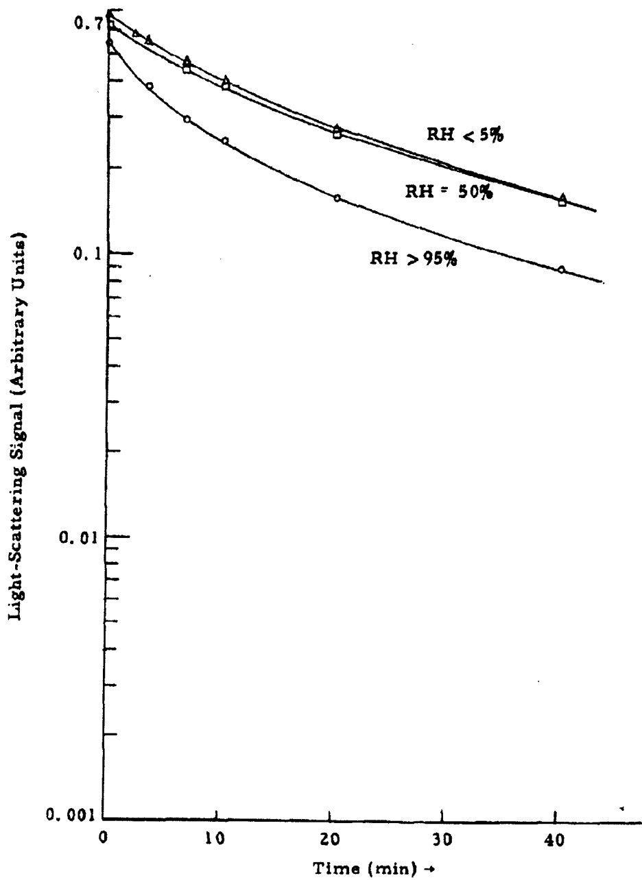
Figure 3.2 Effect of Humidity on Decay of Saccharin Aerosols ( \approx 57 mg Samples)
