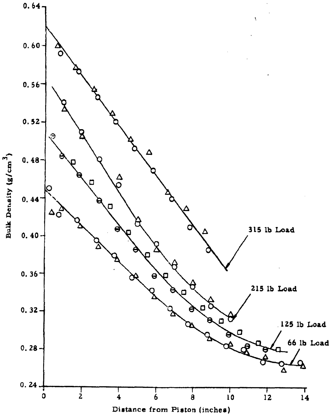
Figure 2.20 Bulk Density of Talc (Mistrion Vapor) as a Function of Distance from Piston at Various Compressive Loads
