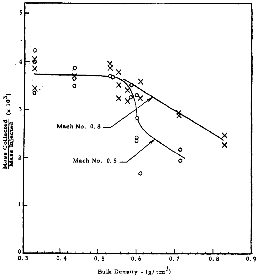
Figure 4.1 Concentration of Fine Sm Aerosol Cloud in Wind Tunnel as a Function of Bulk Density - Sampling Probe at 0.5 inches from Wall
