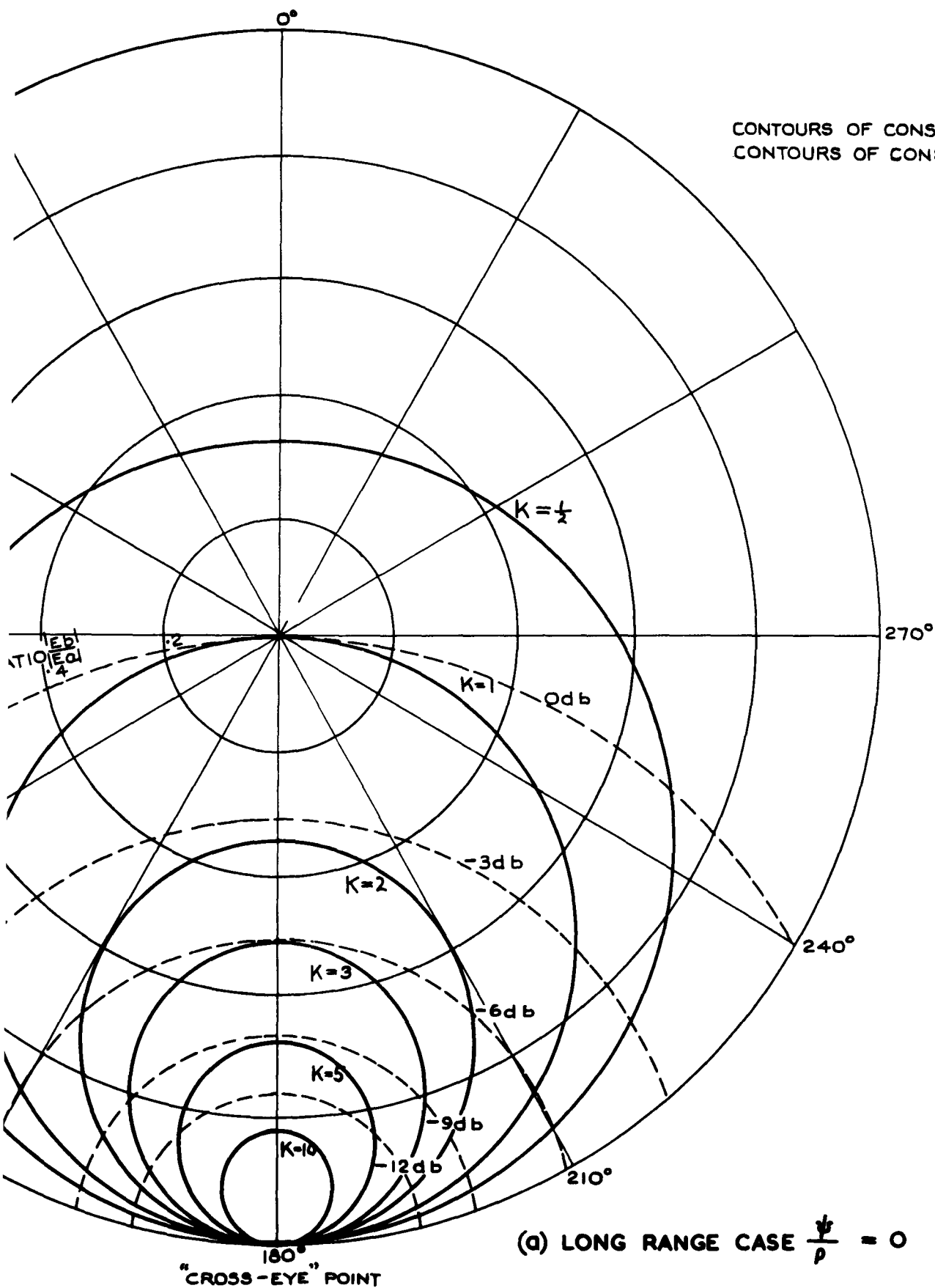
FIG. 3. TRACKER RESPONSE POLAR CHART.
