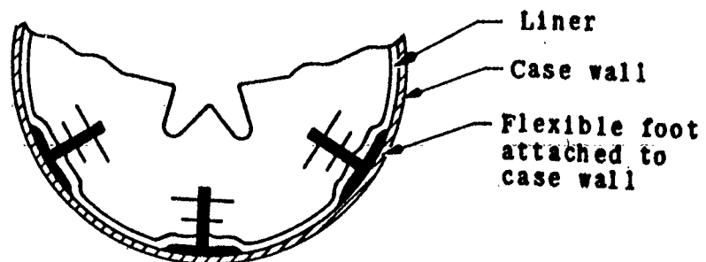
Figure 2. Reinforcement to Reduce Liner Separation.
