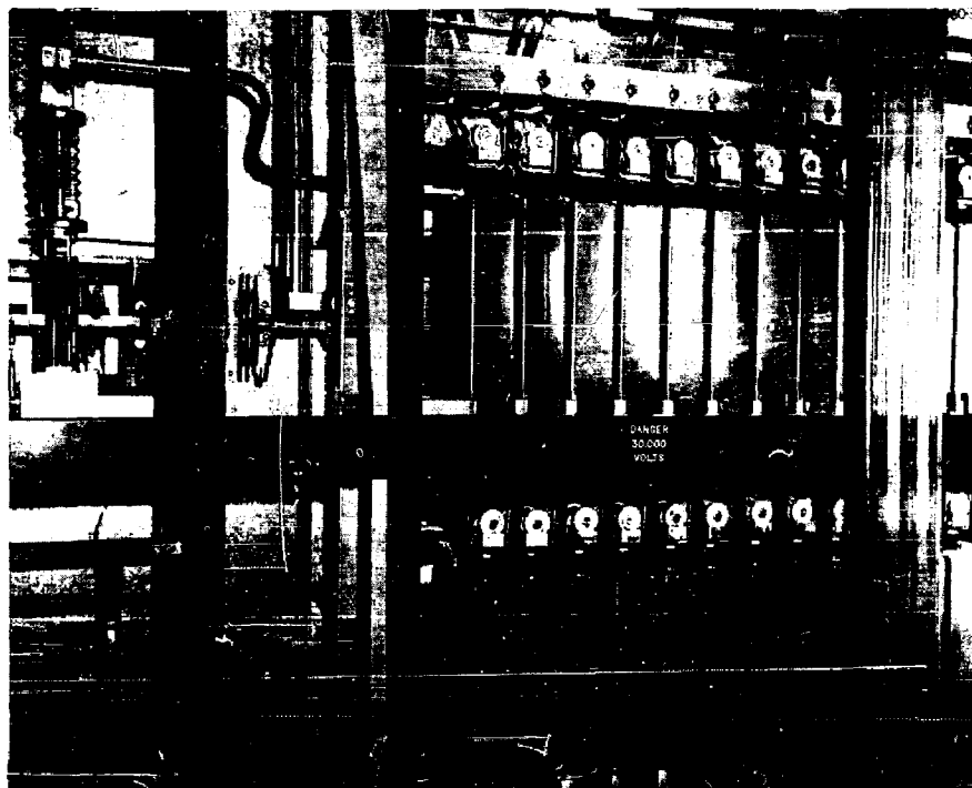
Figure 10 - Capacitor bank, showing a manual safety switch on the left and fuses in series with each capacitor
