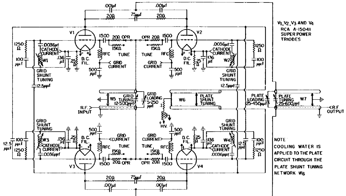
Figure 3 - Schematic diagram of the high-power amplifier (HPA)
