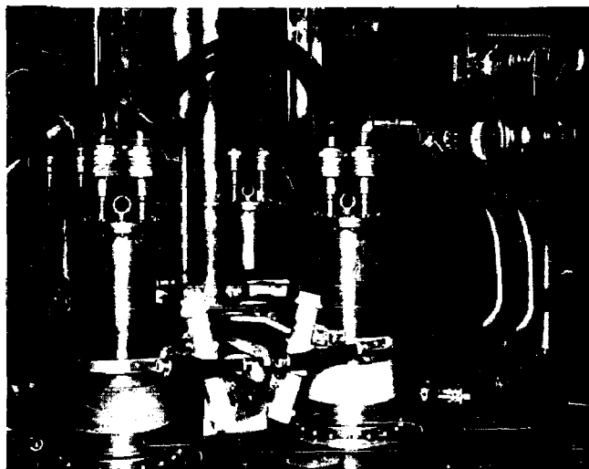
Figure 4 - HPA configuration, top side. The four tubes are visible with their connecting water hoses on top for plate cooling. The plate shunt tuner extends beyond the top of the picture. A series string of neutralizing capacitors is seen in the lower left, while at the upper right can be seen the plate loading and tuning capacitors.
