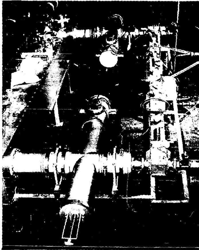
Figure 18 - Duplexer. The high-power contradirectional coupler is on the left, with the lower-power one on the right. In the center are the two tuned coaxial transformers containing the TR tubes.
