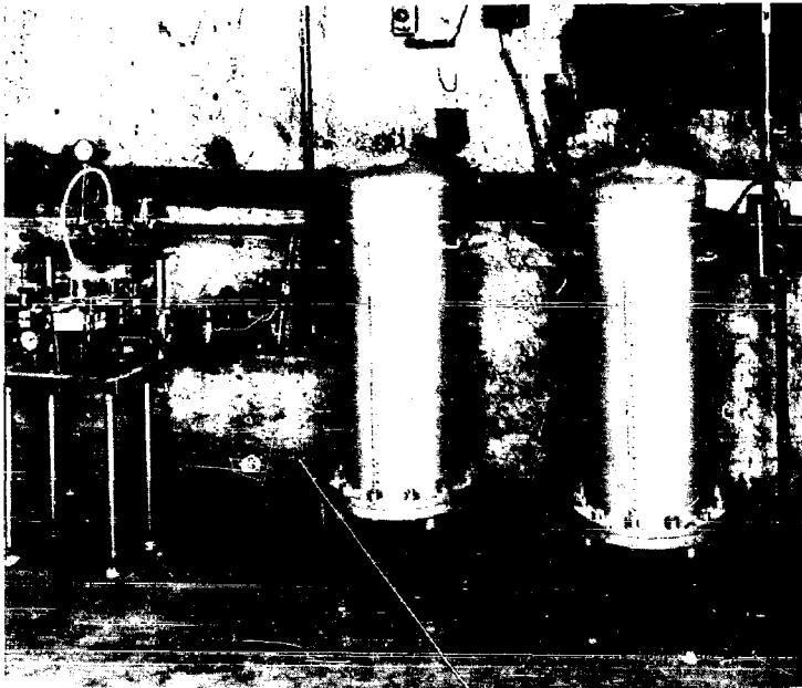
Figure 11 - Tube water-treatment system. The micron filter is on the left, the demineralizer is in the center, and the deoxygenator is on the right.
