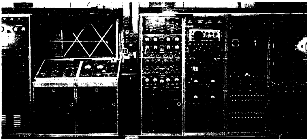
Figure 6 - Control panel and equipment located in front of the HPA shielded room. Arranged from left to right is the grid pulser (two racks), the HPA main control panel (sloping), the HPA tuning rack, the HPA monitor rack, and the two racks for the controls of the two antennas and the antenna monitor.
