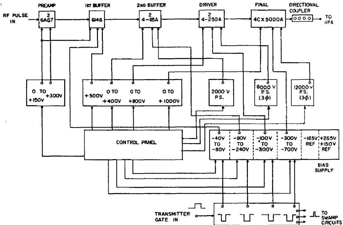
Figure 2 - Block diagram of the intermediate-power amplifier
