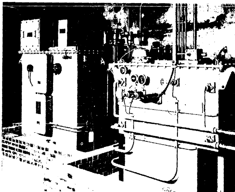
Figure 8 - Water load. The load itself is located in the left center, connected to a 9-in. coaxial switch. The large tube on the right is the water-to-water heat exchanger, while the tank at the top center is the reservoir, which is open to atmospheric pressure.
