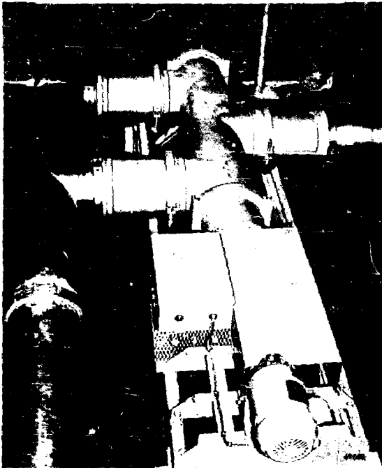
Figure 20 - SPDT 9-3/16-in. coaxial switch. The drive motor is in the lower right; the common arm is on the right.
