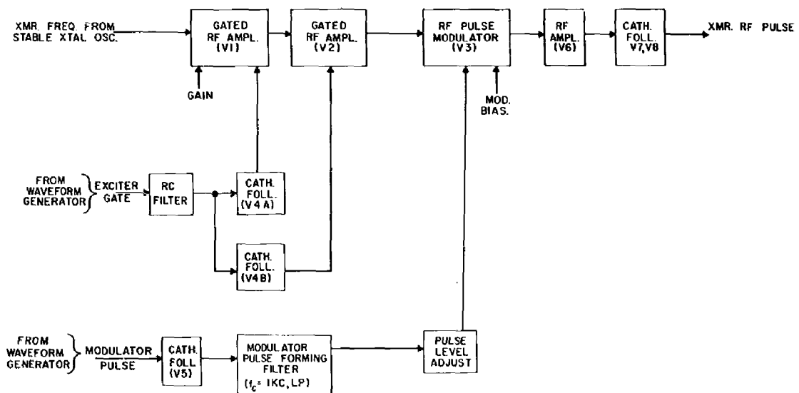
Figure 1 - Block diagram of the exciter
