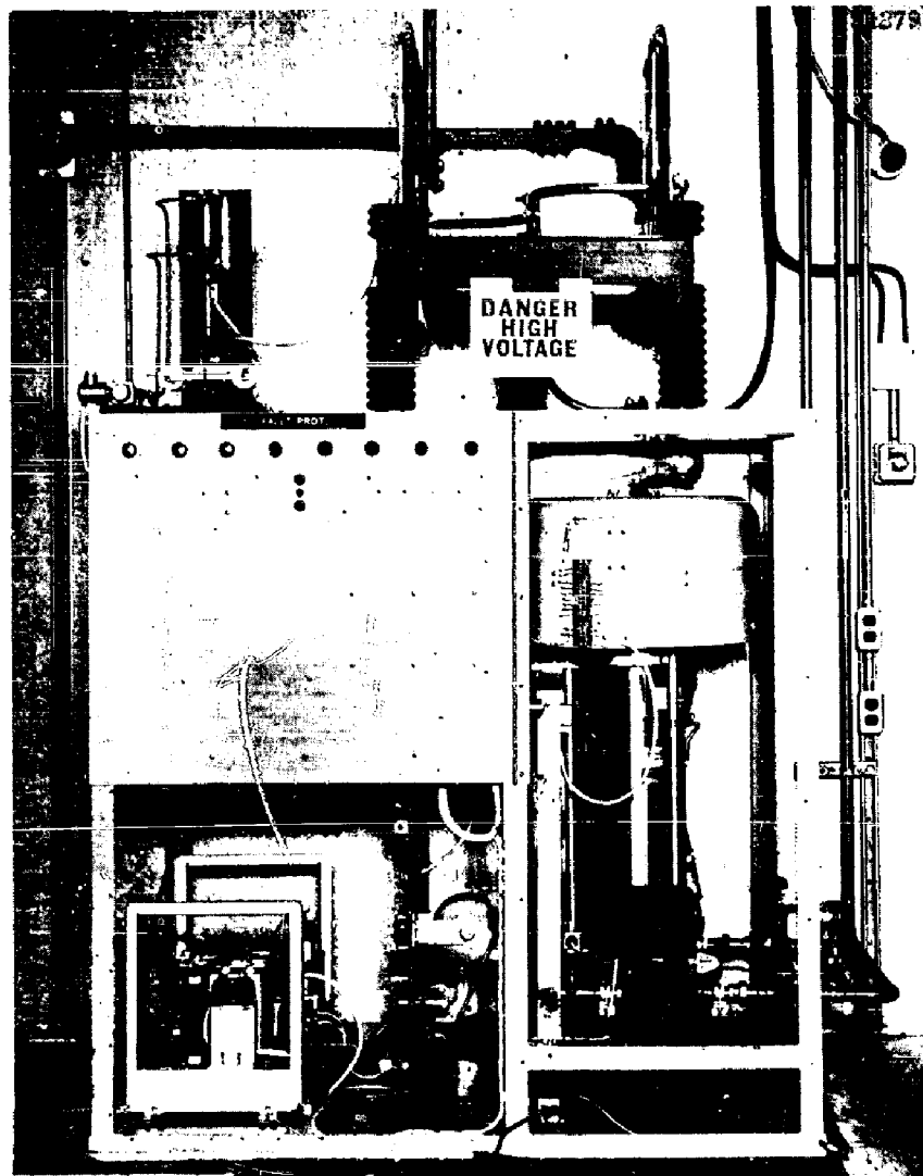
Figure 17 - Electronic "crowbar" fault protector. The ignitron is located on the right-hand side of this unit.
