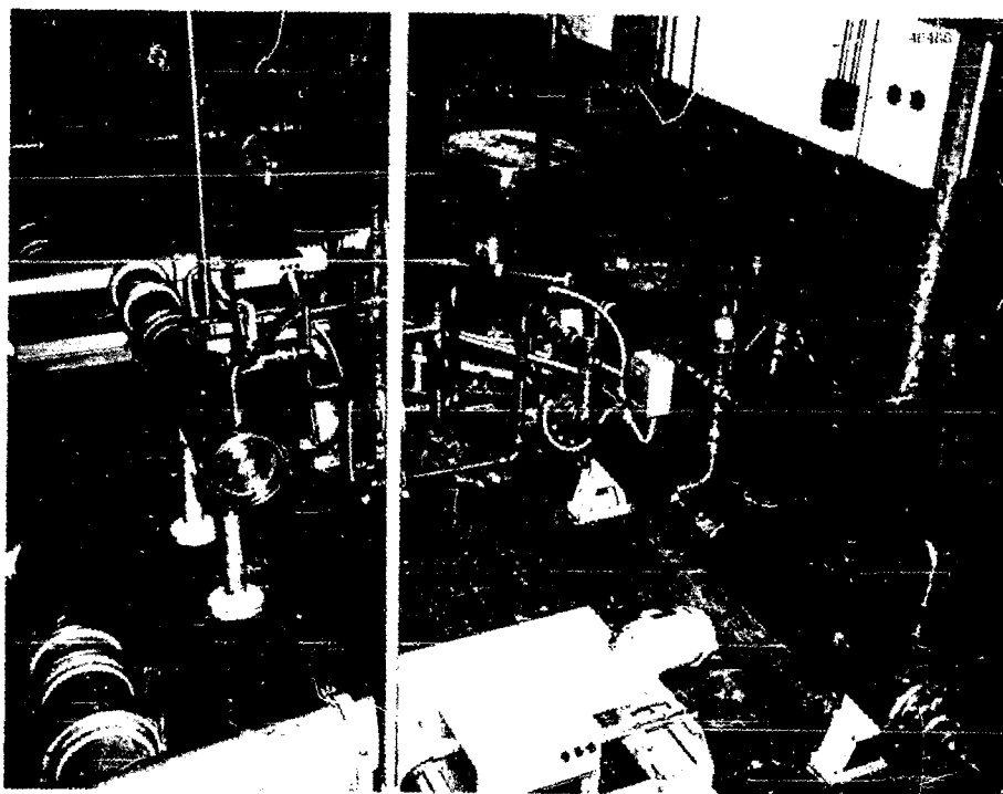
Figure 8 - Water load. The load itself is located in the left center, connected to a 9-in. coaxial switch. The large tube on the right is the water-to-water heat exchanger, while the tank at the top center is the reservoir, which is open to atmospheric pressure.
