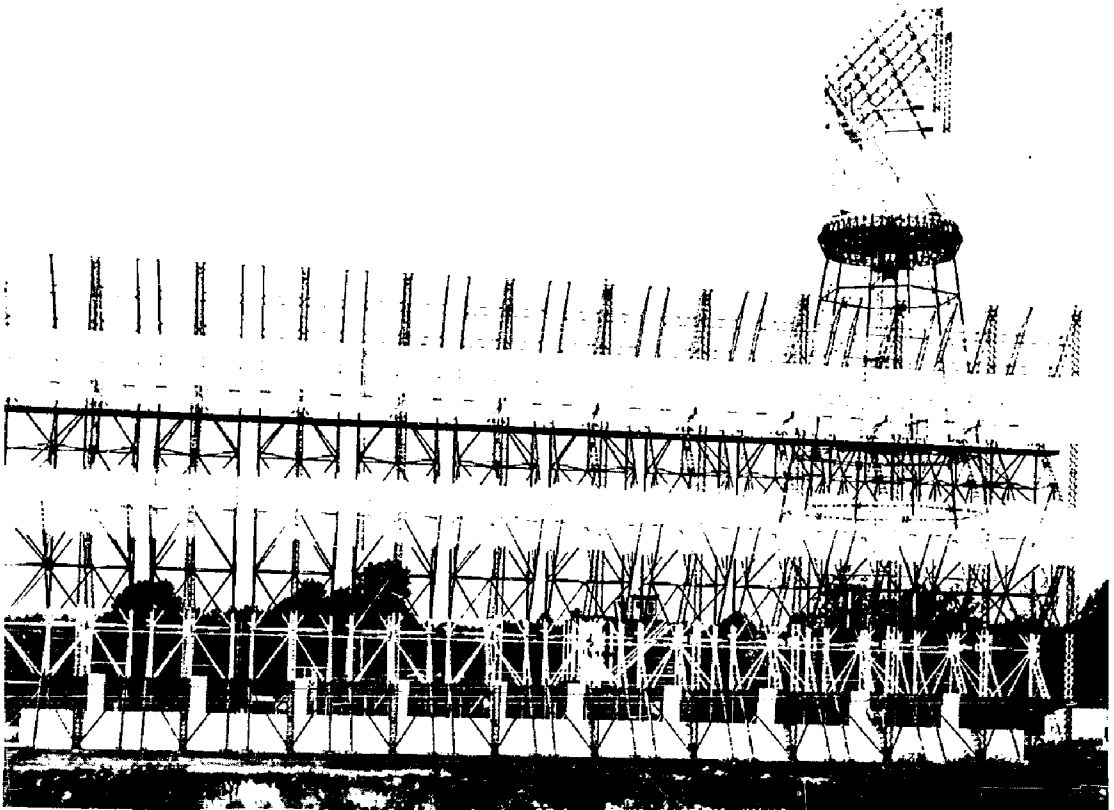
Figure 23 - Front view of the antennas. The fixed antenna is 330 ft long by 140 ft high. Behind it may be seen the positionable antenna, mounted on a 180-ft tower.
