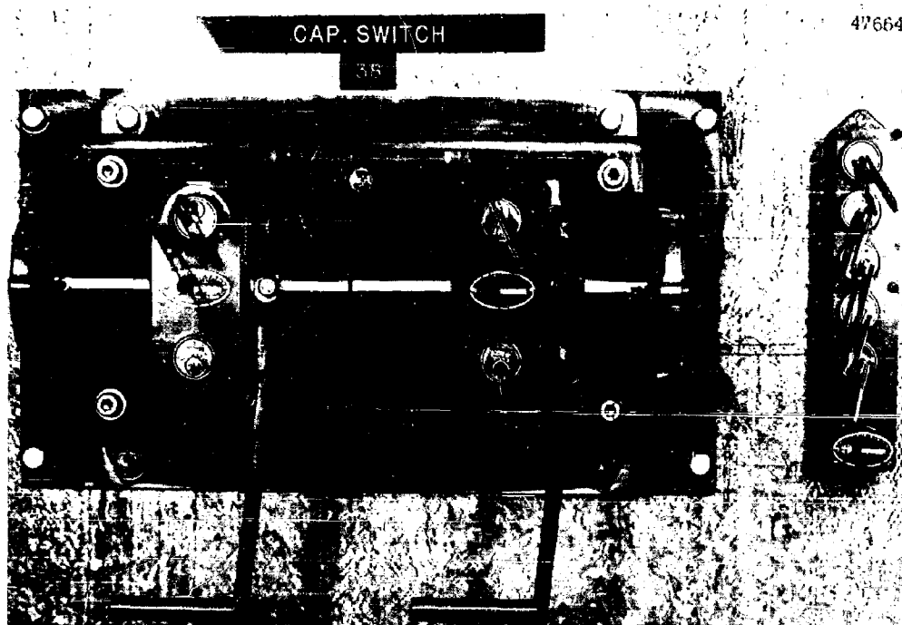
Figure 16 - Key interlock system. The large switch on the left discharges the filter capacitors through a resistance, then the large switch to the right places a short circuit across the filter.
