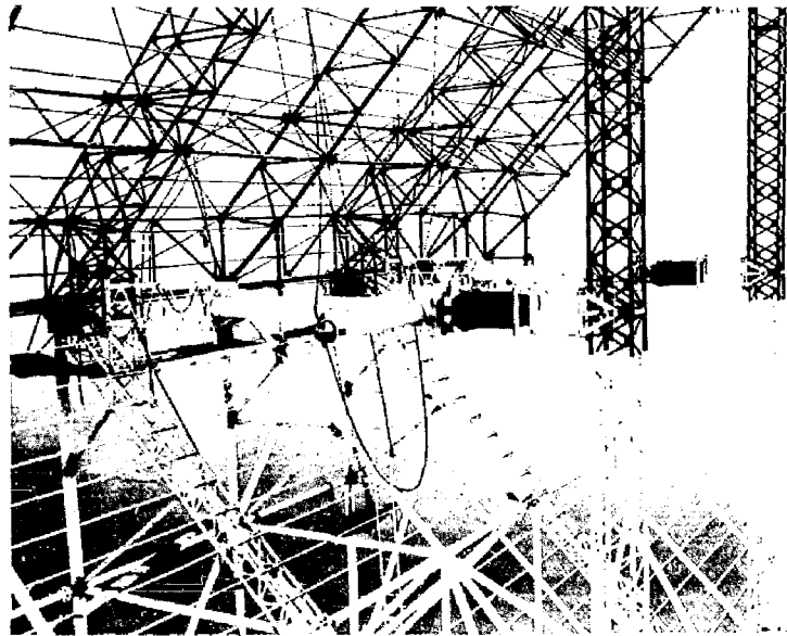
Figure 27 - Close-up of positionable antenna, showing dipoles
