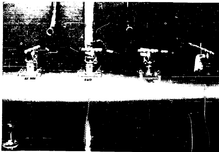
Figure 21 - Directional couplers for rf monitor. Appearing from left to right, the couplers are used as follows: power-output indicator, forward power, reflected power, and reflected-power fault sensing.
