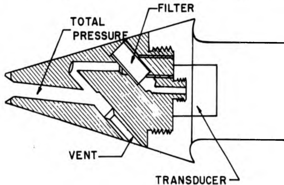
Figure 3.2 SRI supersonic total-head gage.
