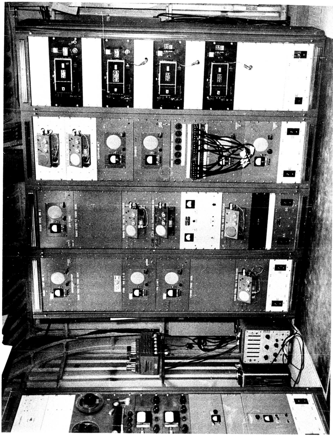
Fig. 2.4 - Radio and Bhangmeter racks
