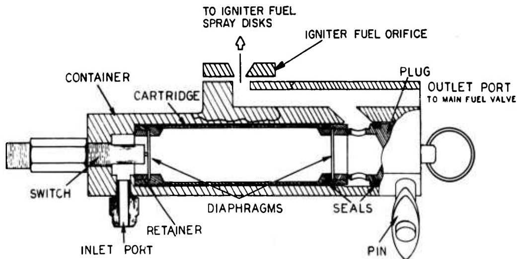
FIG. 15 HYPERGOL CONTAINER
