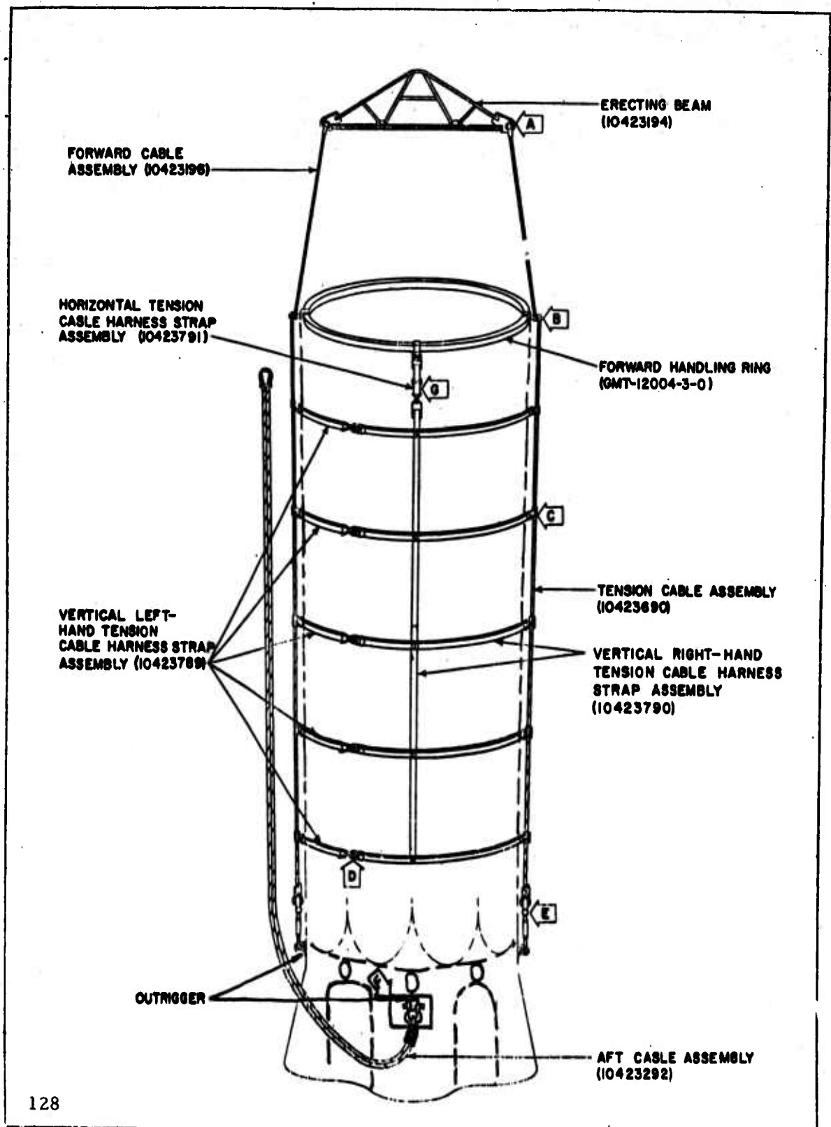
FIG. 54 ERECTING KIT DETAILS
