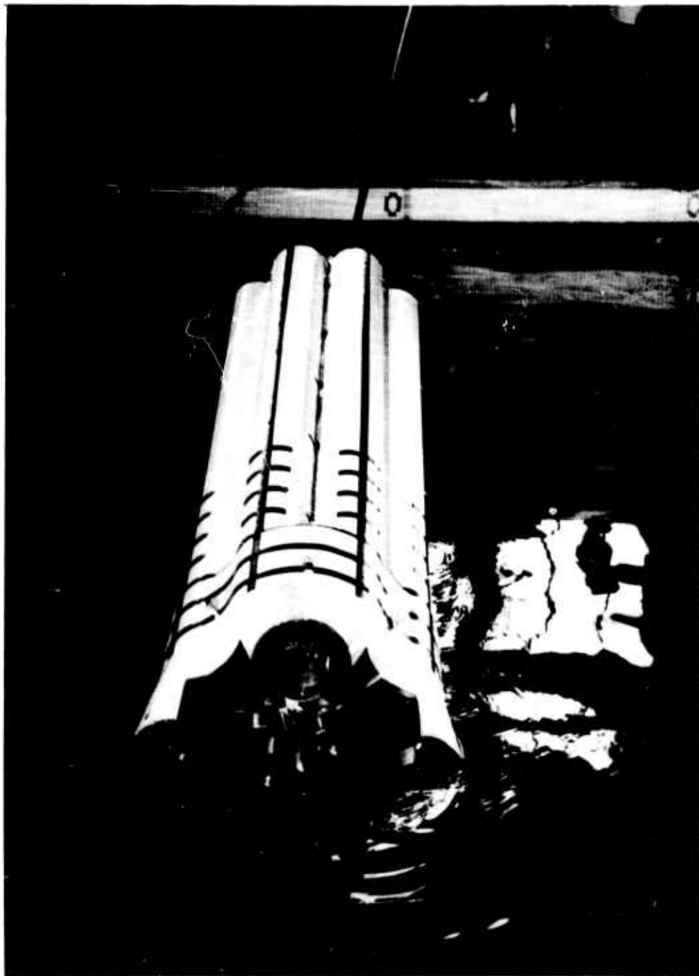
FIG. 79. ONE-TENTH SCALE MODEL IN THE WATER - END VIEW
