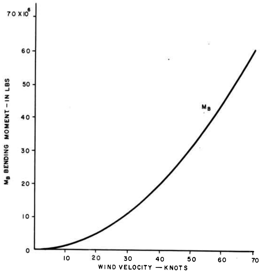
ON LAUNCHER FIG. 6. BENDING MOMENT VS WIND VELOCITY
