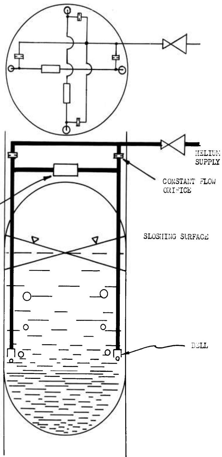
TUBING ARRANGEMENT FOR SLOSHING MEASUREMENT
