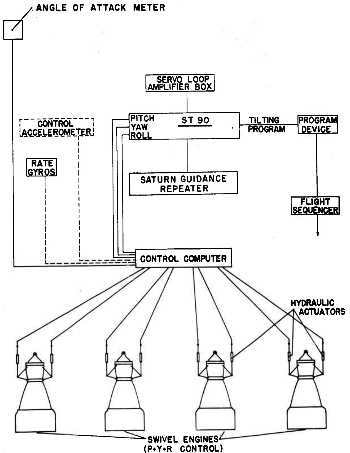
FIG. 24. BOOSTER CONTROL SYSTEM
