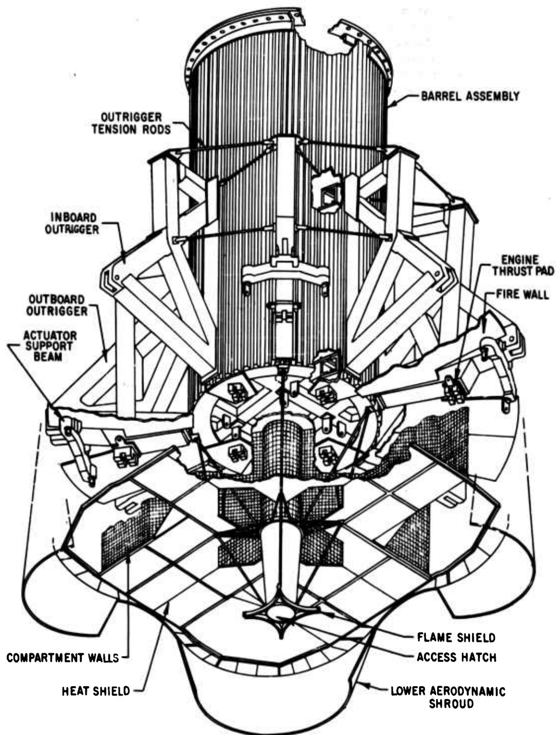
FIG. 2 TAIL SECTION ASSEMBLY SATURN BOOSTER
