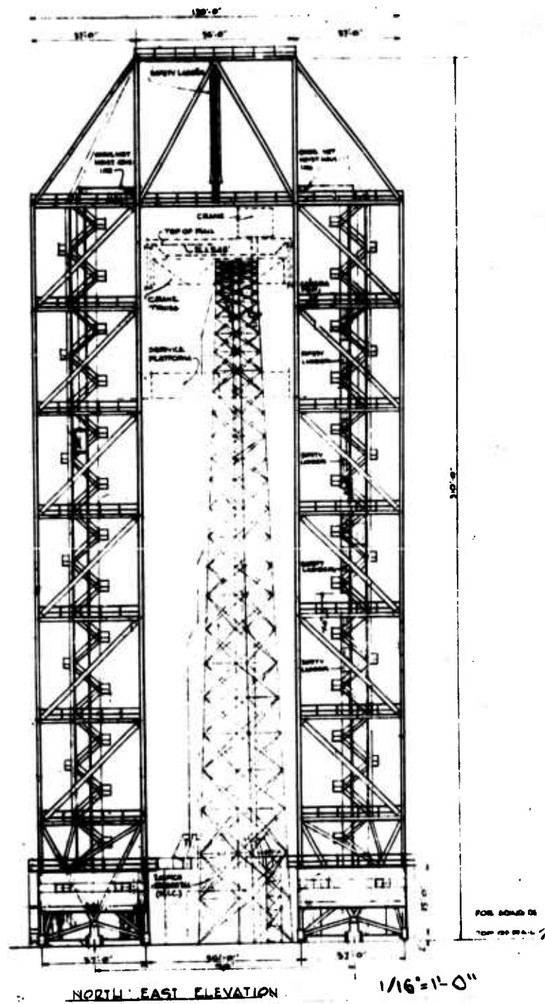
FIG. 73. SERVICE STRUCTURE
