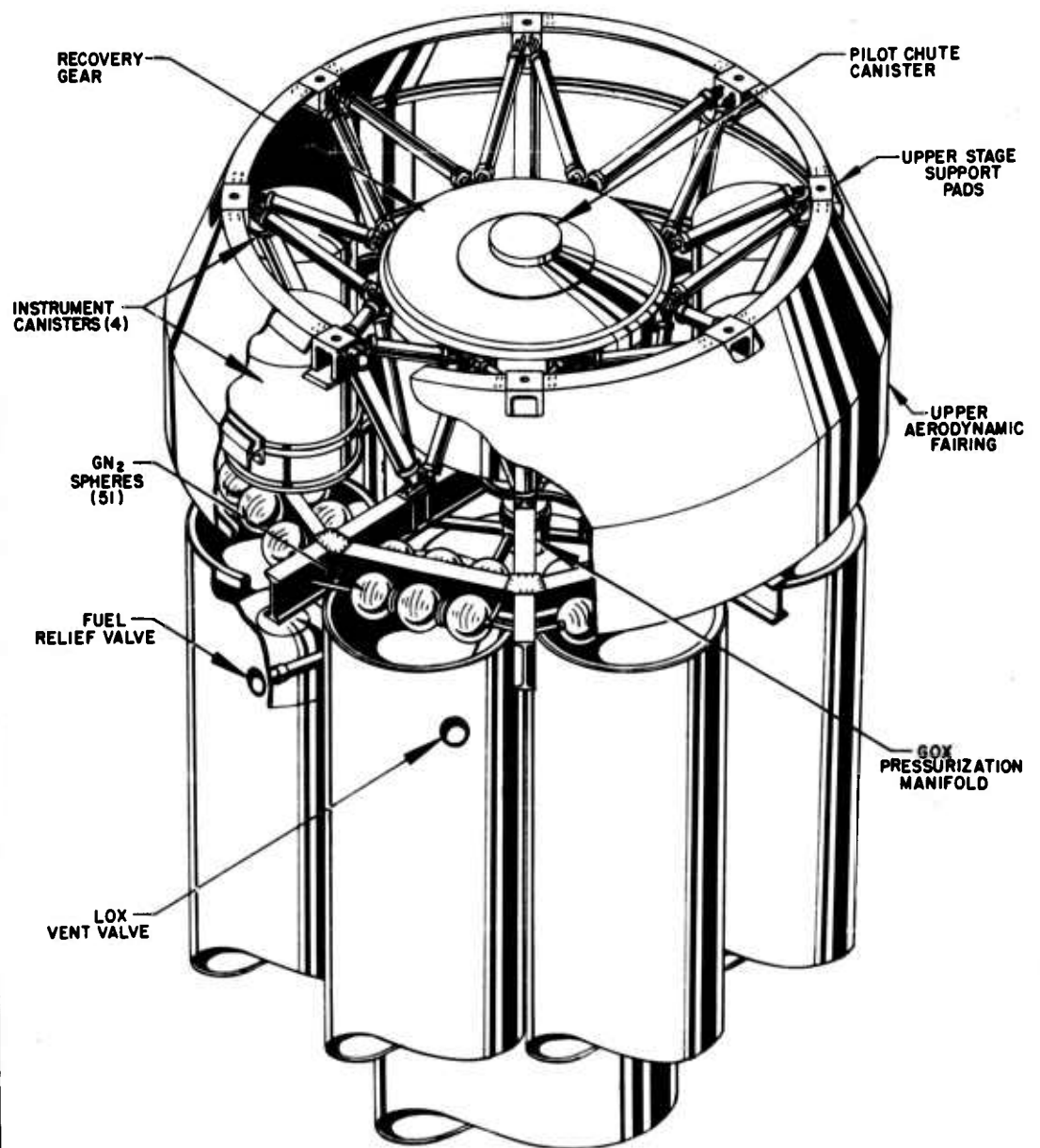
FIG 4 UPPER STAGE ADAPTER AREA SATURN BOOSTER
