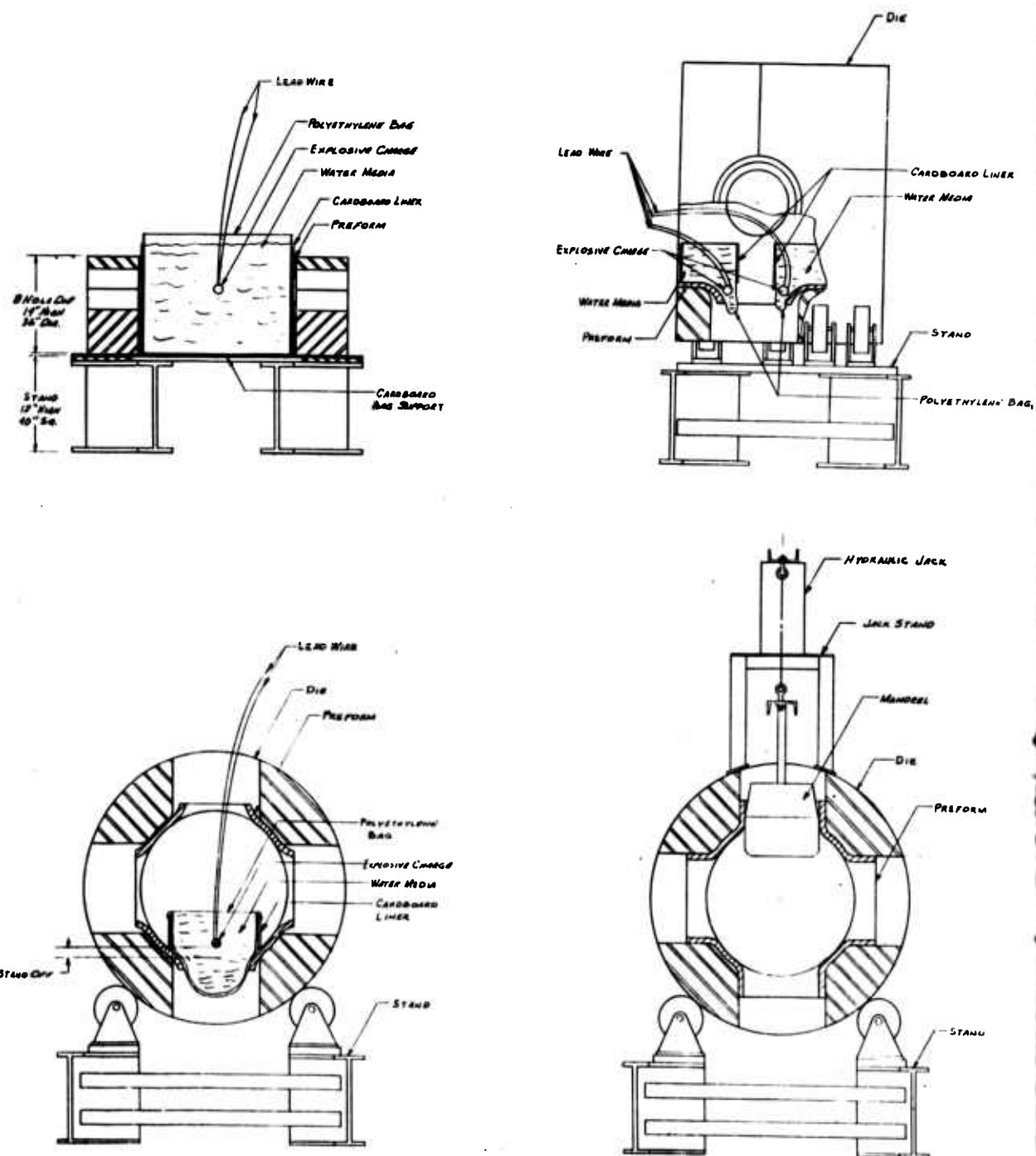
FIG. 41. EXPLOSIVE FORMING PROCESS
