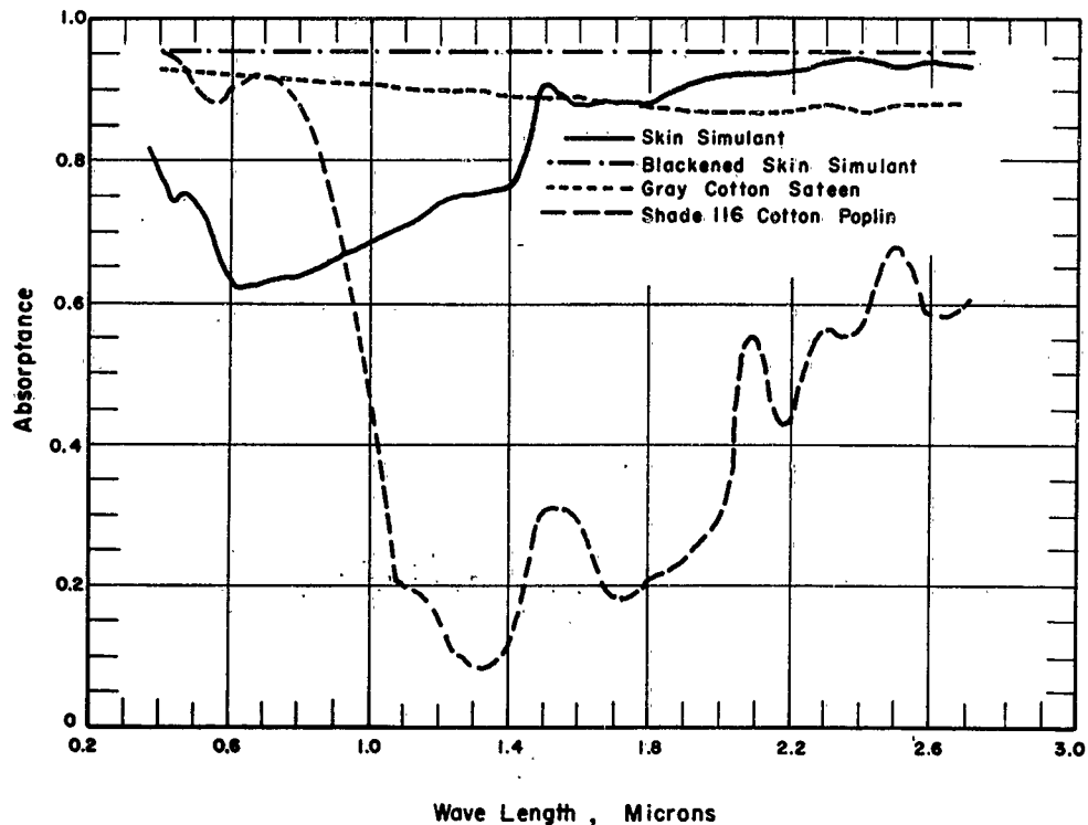
Figure 1.1 Spectral absorptances of NML skin simulant and standard fabrics.
