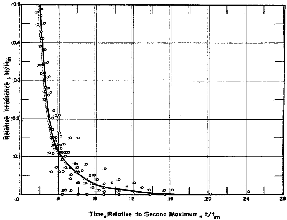
Figure 2.5 Decay portion of irradiance history, Shot Yellowwood.
