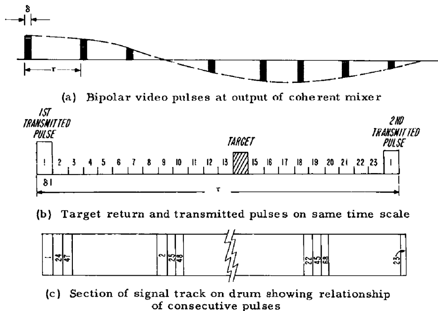
Fig. 2 - Time and space relationships of pulses in the system
