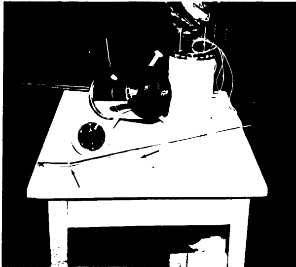
Fig. 1 - Fractured 20-inch satellite components after failure at 20 g and 44 cps; arrows indicate points of failure
