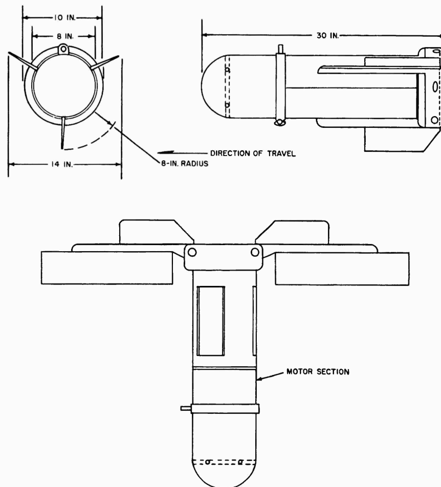
FIG. 30. Motor Package for the 8-Inch Cyclops II.
