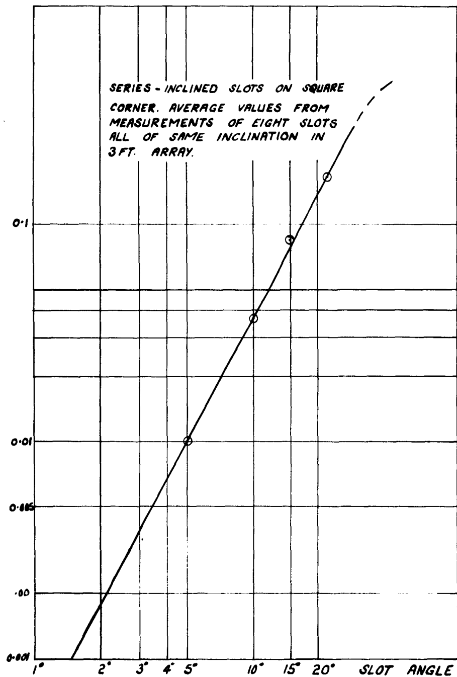
FIG. 15. NORMALIZED CONDUCTANCE OF SINGLE SLOTT AGAINST ITS ANGLE OF INCLINATION
