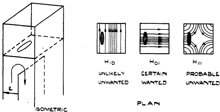
FIG 4 MODES OF RADIATION FROM A SQUARE WAVEGUIDE HORN EXCITED BY SHUNT-DISPLACED SLOT
