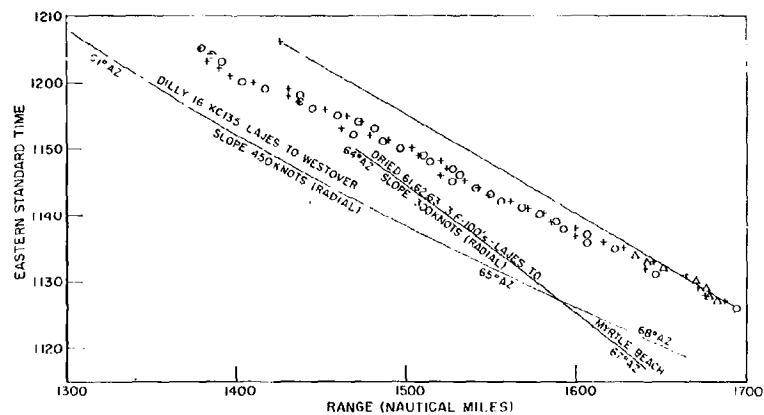
Fig. 9a - Target observed with a relative radial speed of 402 to 418 knots; antenna azimuth, 71 degrees
