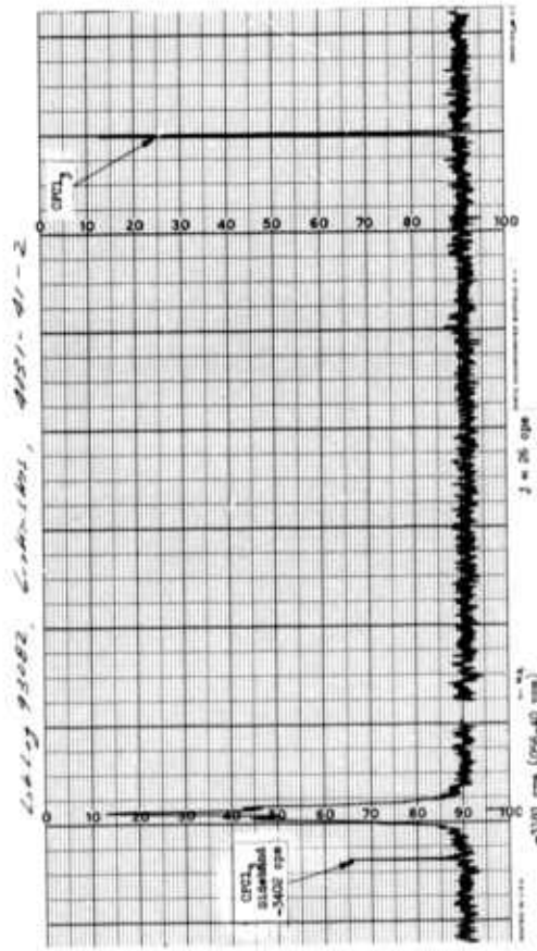
Fig. 35 Fluorine NMR Spectrum of Ethyl Difluoroaminoacetate
