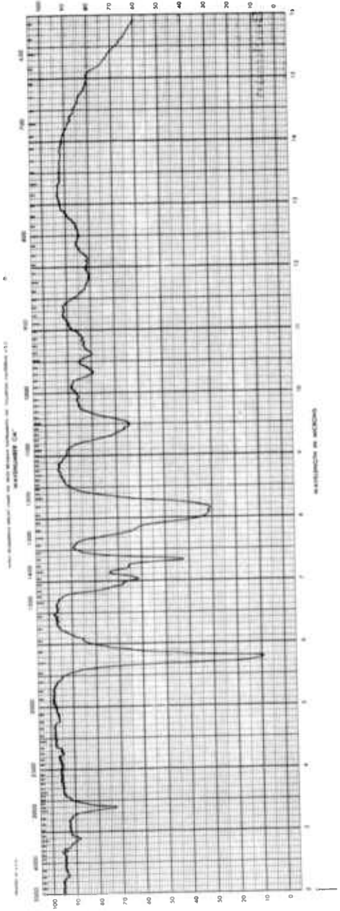
Fig. 24 Infrared Spectrum of beta-Difluorinoethyl Acetate
