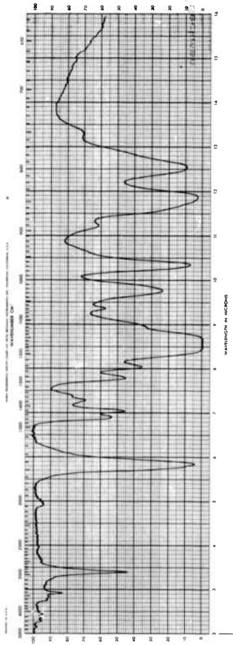
Fig. 29 Infrared Spectrum of \beta -Difluoroaminoethyl Formate
