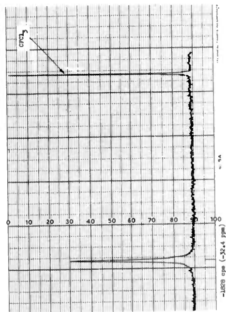
Fig. 37 Fluorine NMR Spectrum of Ethyl N,N-Difluorohydroxyacetate
