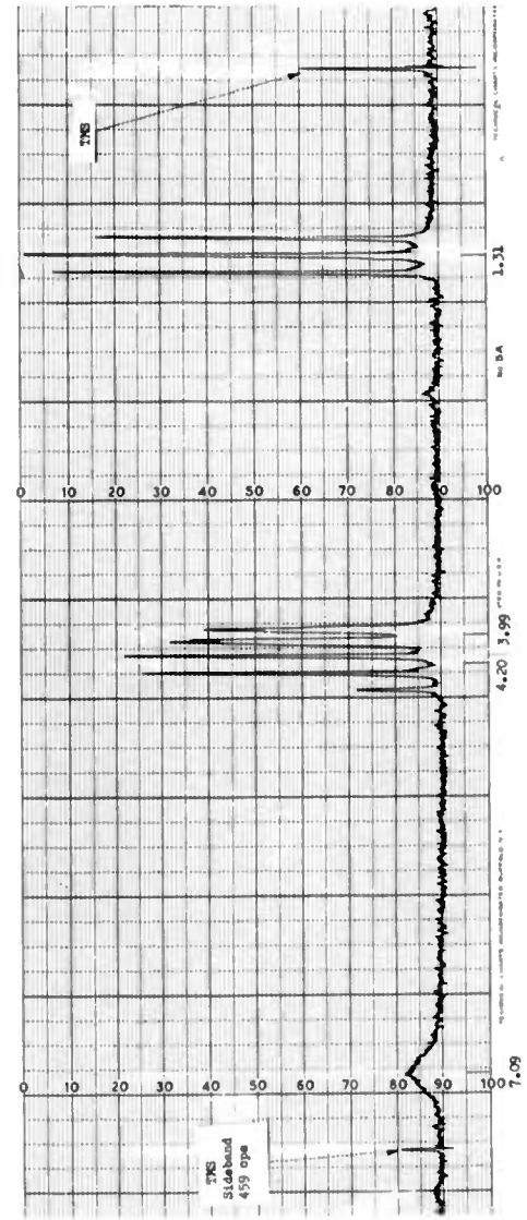
Fig. 36 Proton NMR Spectrum of Ethyl N,N-Difluoroaminoacetate
