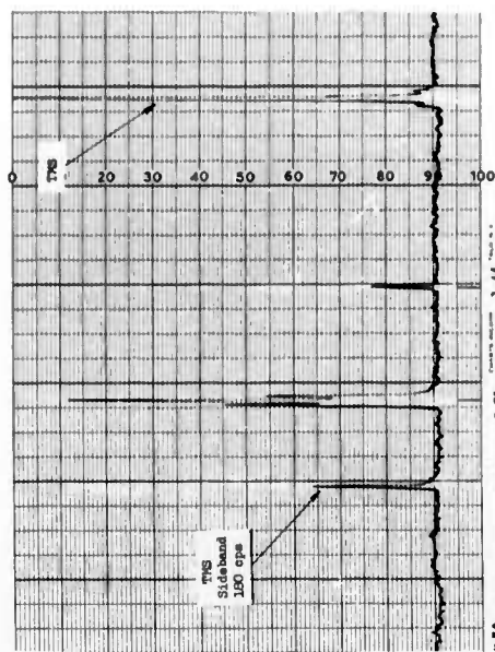
Fig. 2 Proton NMR Spectrum of 1,1-Dichloro-1-(difluoramino)ethane
