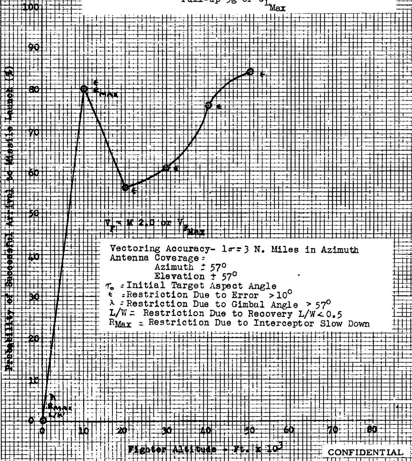
Fig. 64- Probability of Successful Arrival to Missile Launch for CONFIDENTIAL Pull-up Attacks, Head-on - AN/APQ-72 (XN-3) Radar Mach 1.6 Target 50,000 Ft. Pull-up 3g or C_{L_{Max}}
