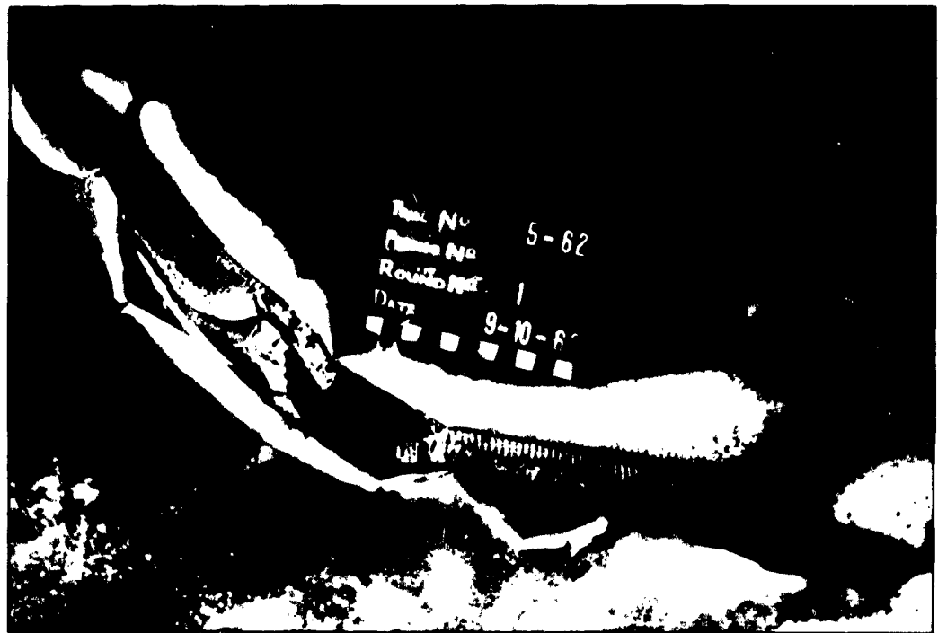
FIG.28c. TARGET 8. ROD DAMAGE TO HONEYCOMB CORE AND INNER SKIN (LOW VEL. \frac{1}{8} in. ROD)
