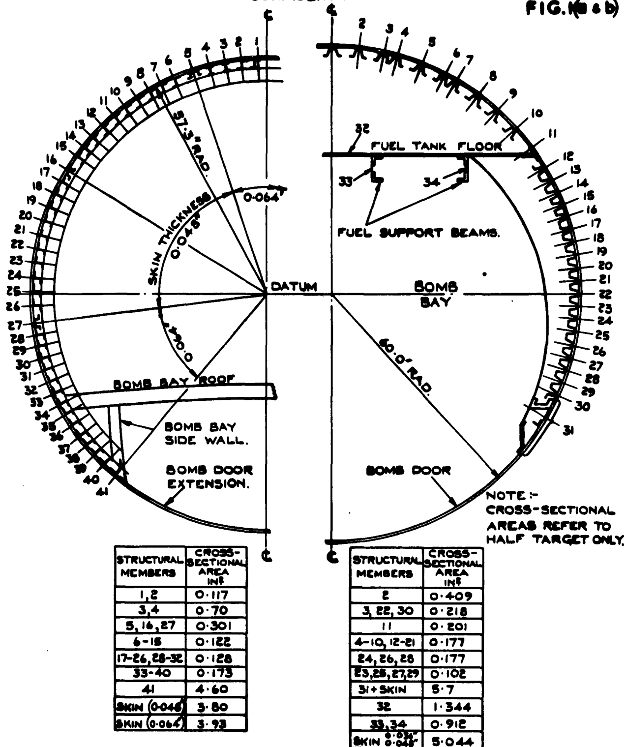
1 (a) STN. 963 VICKERS 'VALIANT' TYPE 673 (TARGET 1A)
