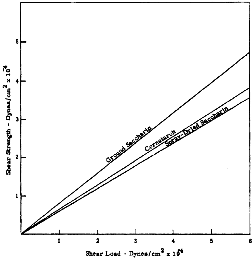
Figure 2.21 Compaction Shear Strength of 12-Micron Powders
