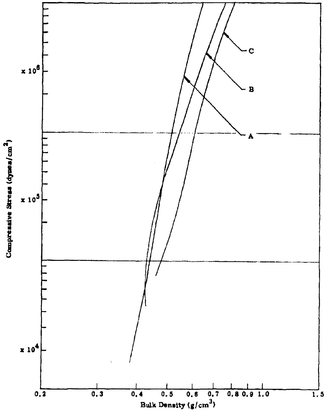
Figure 2.17 Compaction Characteristics of Dried Sm 342 2-23
