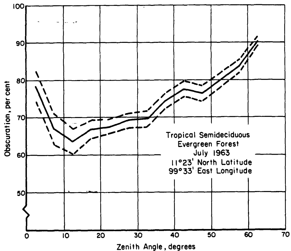
FIGURE 47. EXAMPLES OF MRDC FOLIAGE-OBSCURATION DATA
