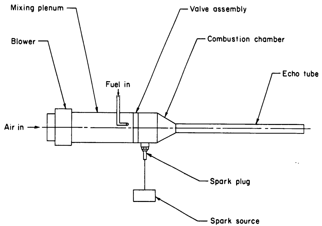
FIGURE 7. HIGH-INTENSITY SOUND GENERATOR
