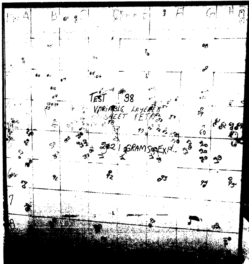
Figure 129. Impact Pattern, Round No. 38
