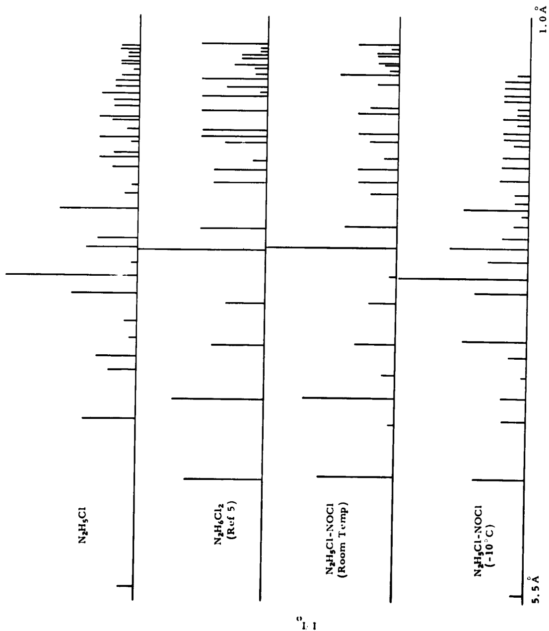
Figure 4. X-ray Diffraction Patterns. Products of N_2H_5Cl-NOCl Reactions
