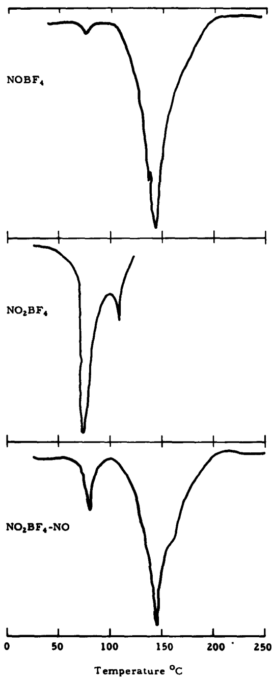
Figure 3. Differential Thermogram of NO- \text{NO}_2\text{BF}_4 Reaction Product
