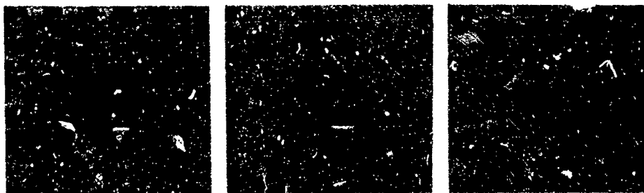
Fig. 6 - Simulated target receding with a doppler frequency of about 40 cps. (a) Conventional Madre radar system primary display, (b) the same receiver, converter, data processing, and display channel with the LSB magnetostriction filter inserted before the synchronous detector, (c) the HSB filter replaces the LSB filter. Horizontal scales represent the range (mi), right-hand scales represent the doppler frequency (cps), and the left-hand scales are not applicable.
