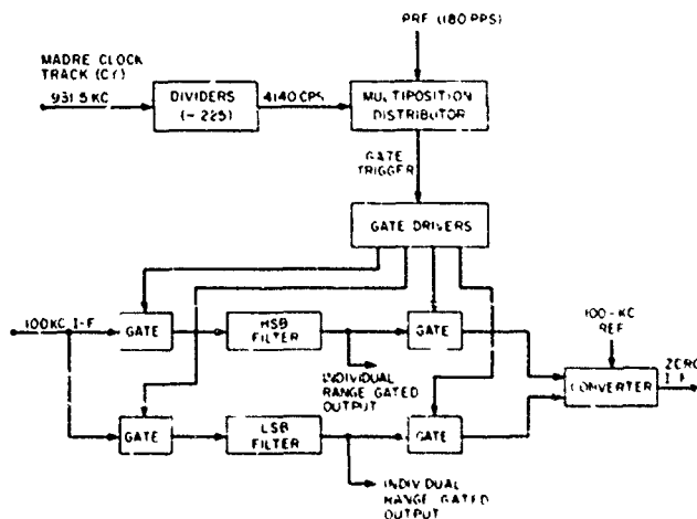
Fig. 1 - Experimental equipment and circuits used to separate approach and recede radar targets by the use of doppler information in the Madre radar system
