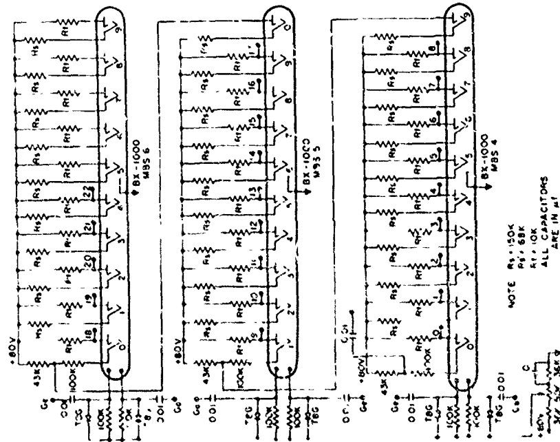
Fig. 3 - Multiposition distributor using three Burroughs BX-1000 beam switching tubes
