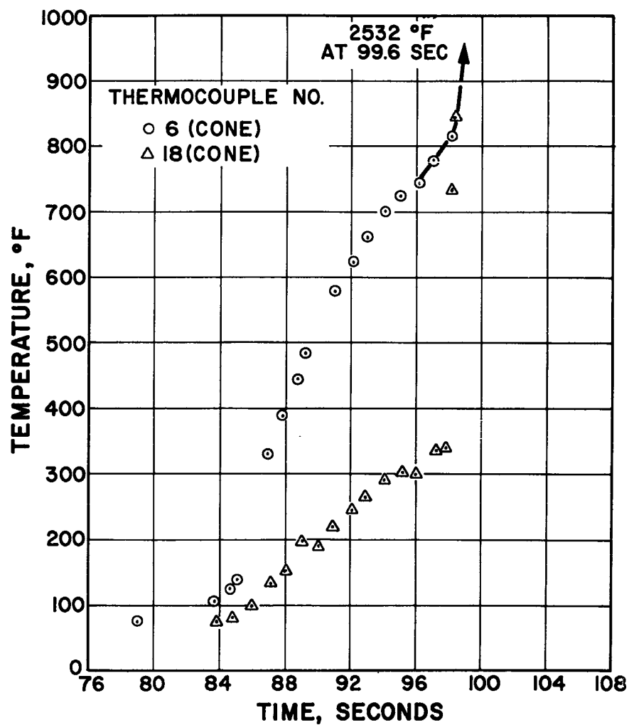
Figure 15. Typical Thermocouple Responses, Flight Two
