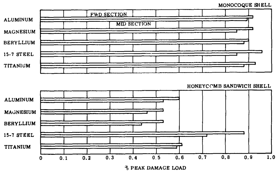
Figure 59. Material Comparison, Vehicle No. 4 ( W/C_D A = 4375 )
