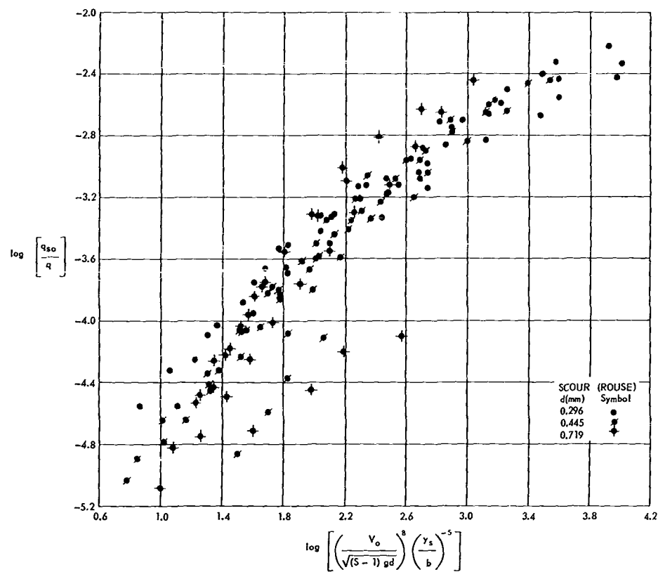
Figure 6. Sediment-Transport Function for Rouse's Minimum Jet Deflection.
